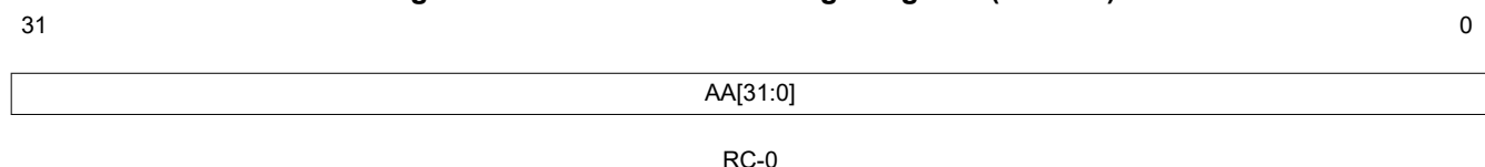
Figure 16-14. Abort-Acknowledge Register (CANAA)
