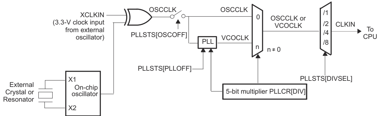
Figure 8-28. OSC and PLL Block Diagram
