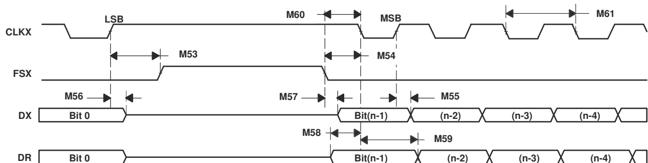
Figure 7-25. McBSP Timing as SPI Master or Slave: CLKSTP = 11b, CLKXP = 1
