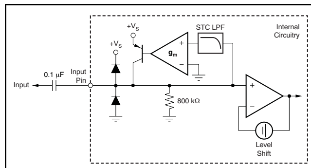
Figure 100. Equivalent AC Sync-Tip-Clamp Input Circuit
