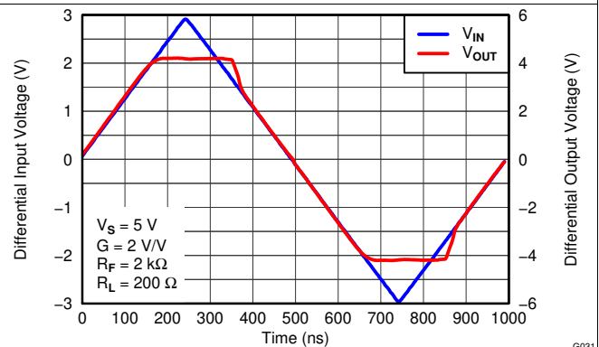
Figure 40. Overdrive Recovery
