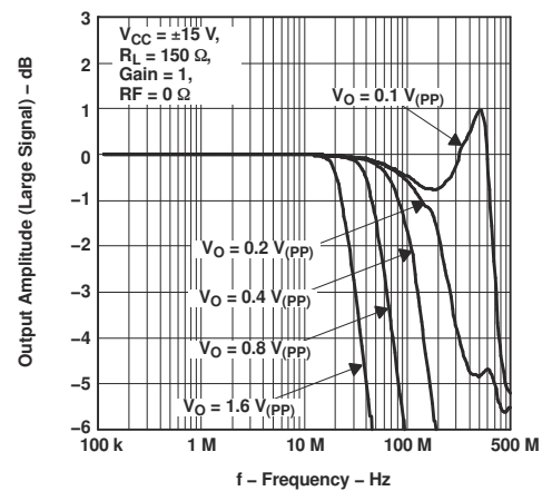
Figure 5-53. Frequency Response With Varying Output Voltage Swing
