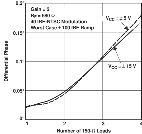
Figure 5-69. Differential Phase vs Number of 150-Ω Loads
