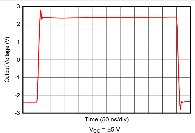
Figure 5-22. 5-V Step Response
