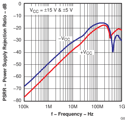
Figure 5-55. Power Supply Rejection Ratio vs Frequency
