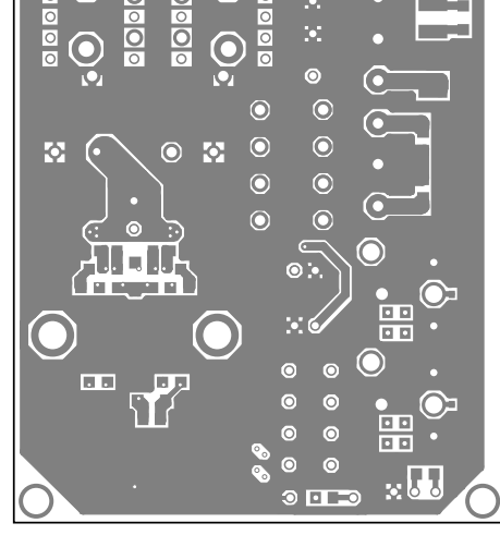
Bottom copper
