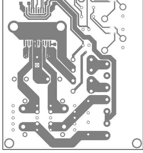
Top copper
