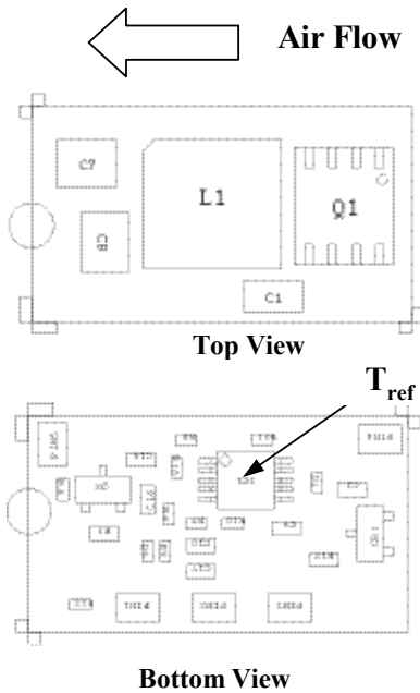
Figure 34. T_{ref} Temperature measurement location.
