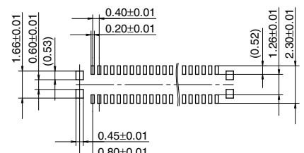
Recommended metal mask pattern Metal mask thickness: When 120μm (Terminal opening ratio: 70%) (Metal-part opening ratio: 100%)
