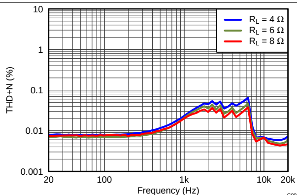
Figure 16. THD+N vs Frequency
