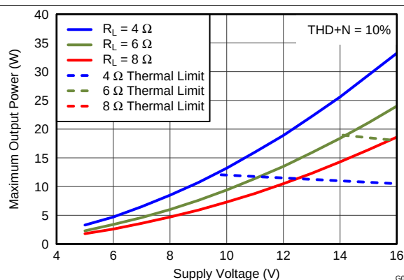
Figure 14. Output Power vs PVDD
