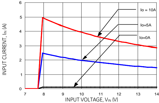
Figure 7. Input voltage vs. Input Current (V out = 3.3Vdc).
