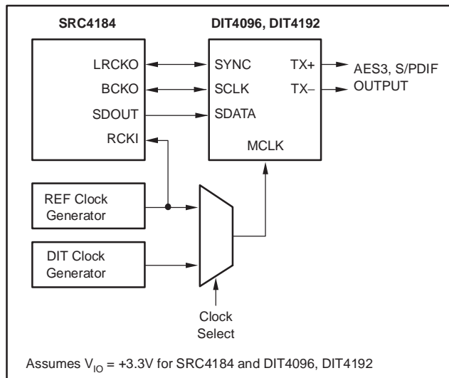
Figure 14. Interfacing the SRC4184 to the DIT4096/4192 Digital Audio Interface Receiver
