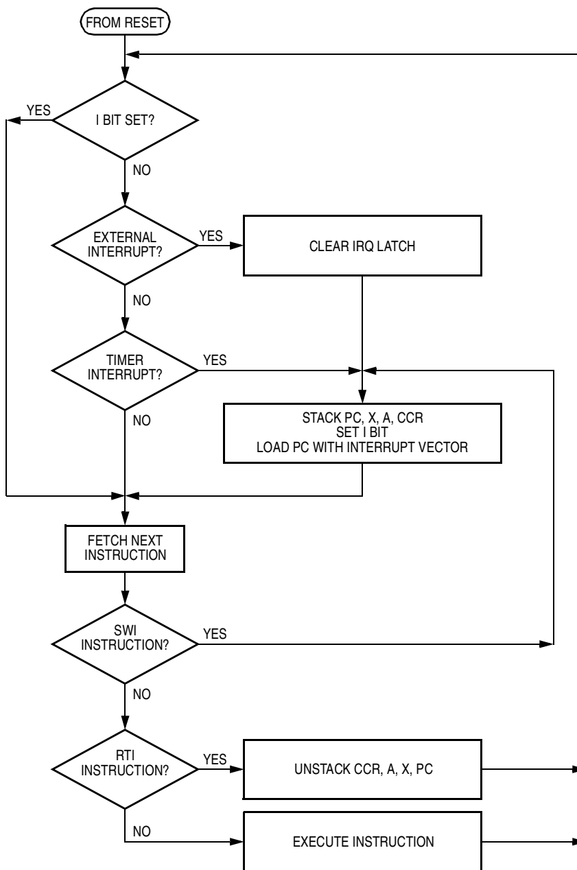
Figure 4-7. Interrupt Flowchart
