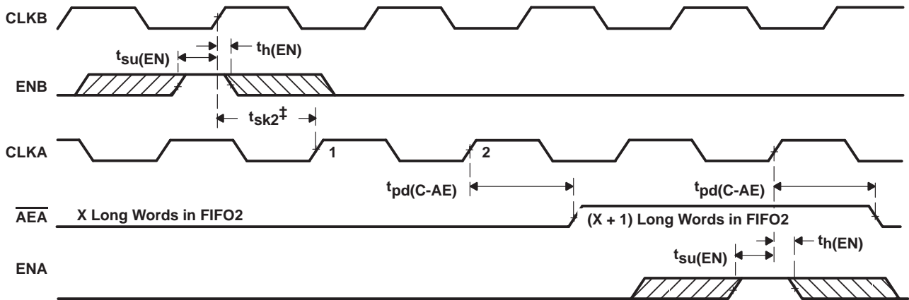
Figure 17. Timing for AEB When FIFO1 Is Almost Empty
