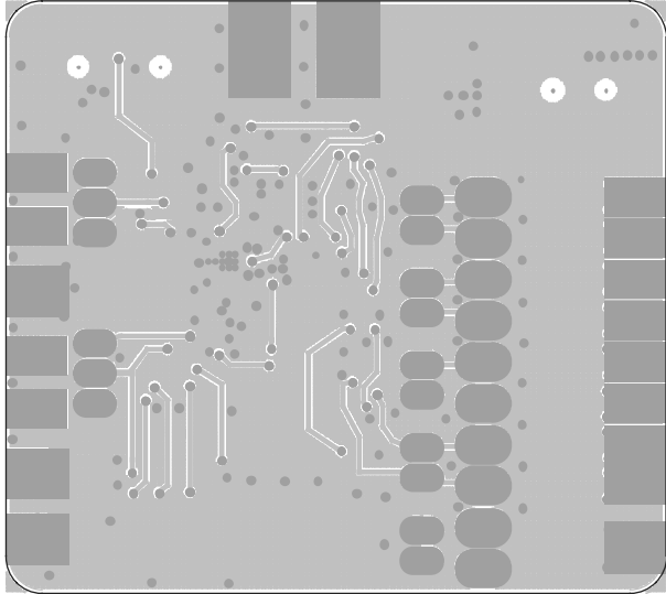
Figure 44. Bottom Layers
