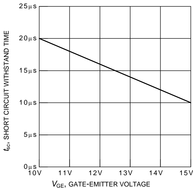
Figure 19. Short circuit withstand time as a function of gate-emitter voltage ( V_{CE} = 600V, \text{start at } T_i = 25^\circ C )
