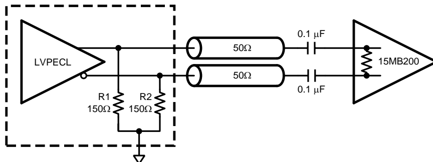
Figure 6. AC Coupled LVPECL to LVDS Interface
