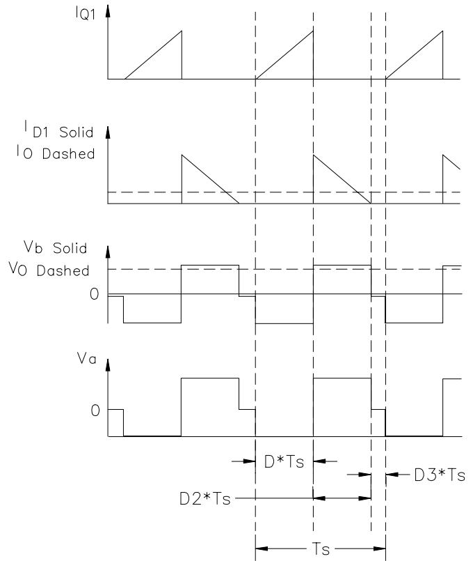
Figure 2: Discontinuous Mode Flyback Waveforms
