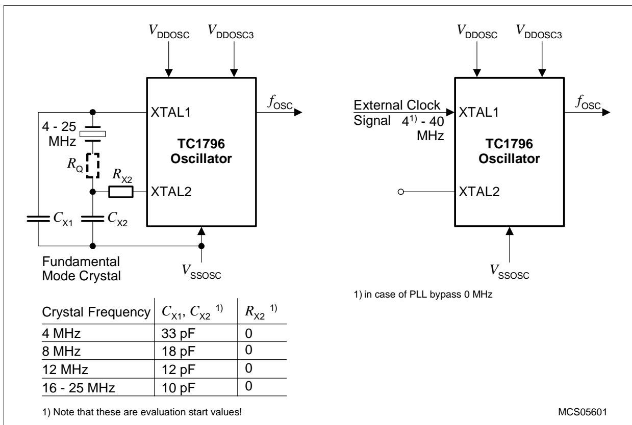
Figure 20 Oscillator Circuitries
