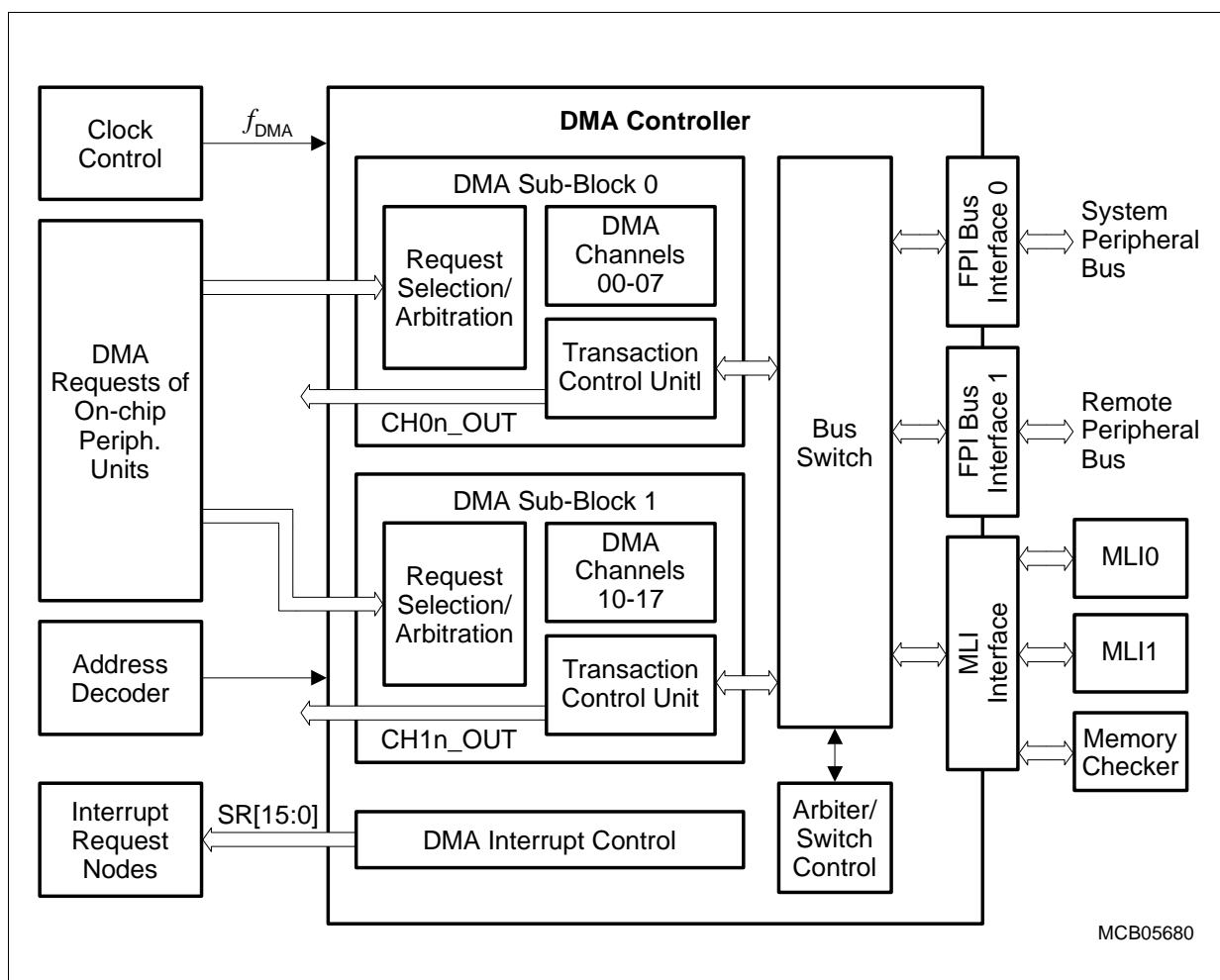
Figure 6 DMA Controller Block Diagram
