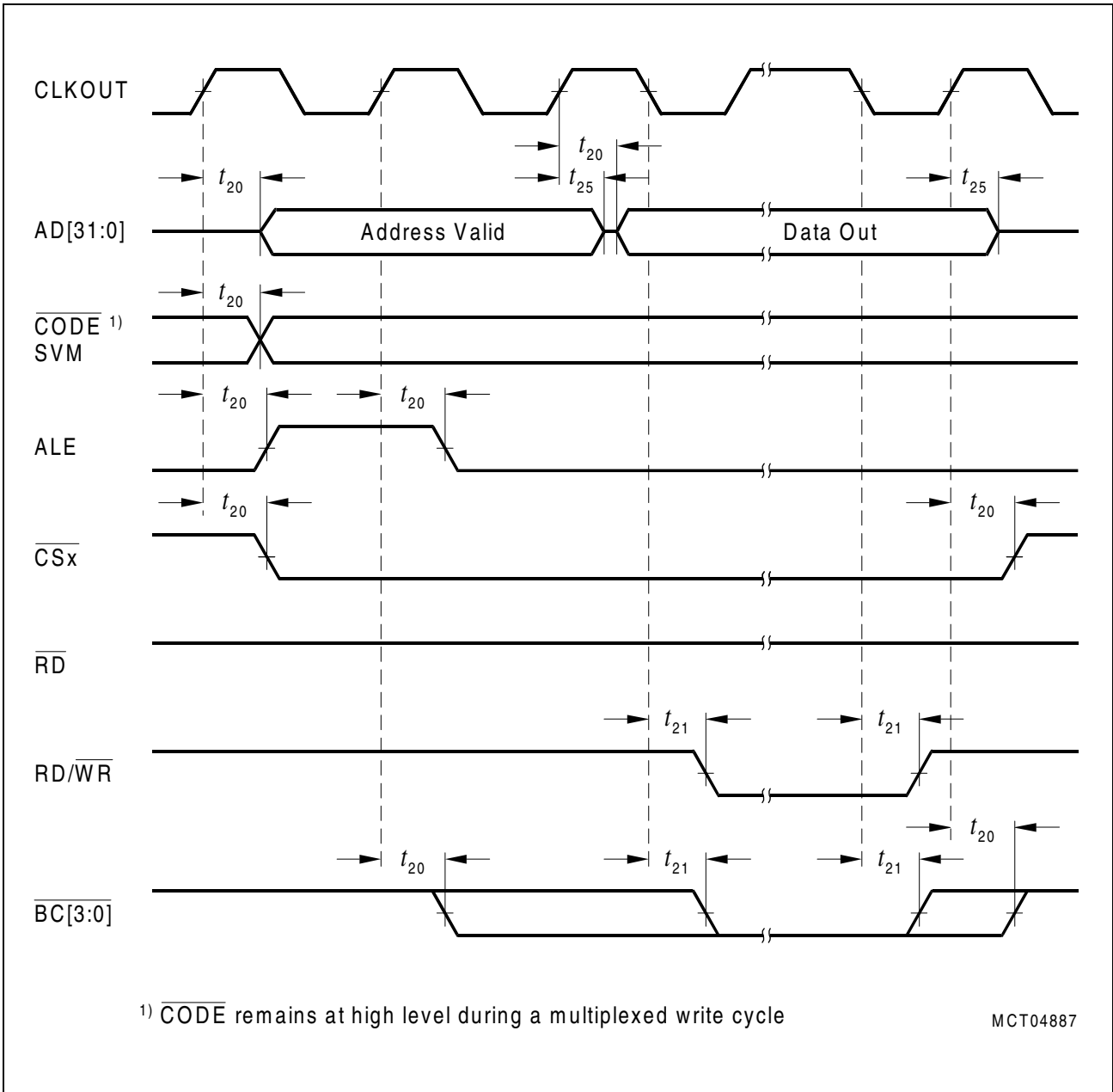
Figure 35 EBU Multiplexed Write Timing
