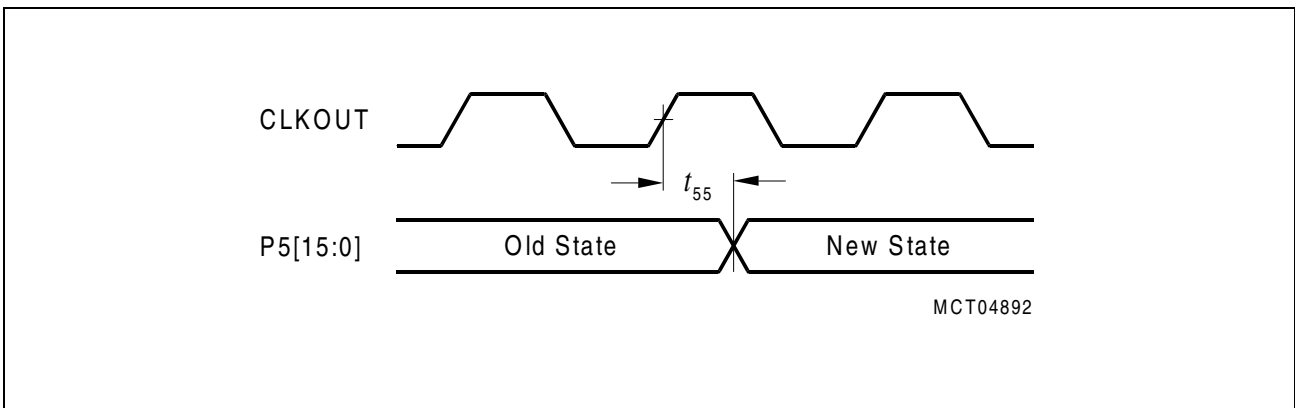
Figure 40 Port 5 Timing
