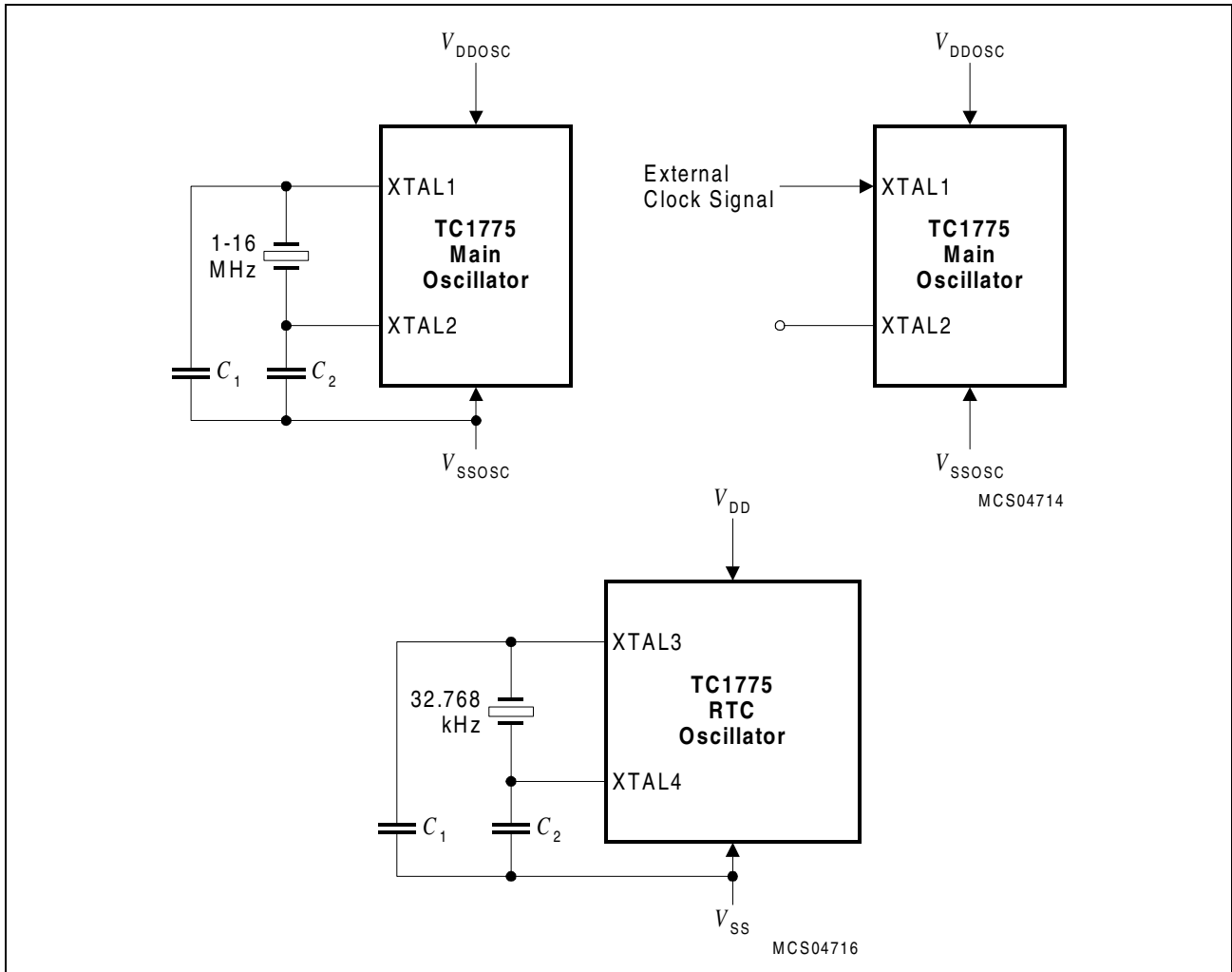
Figure 19 Oscillator Circuitries
