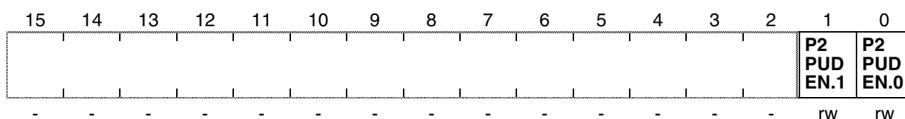
P2PUDEN (FE7A H / 3D H ) SFR Reset Value: - - 00 H
