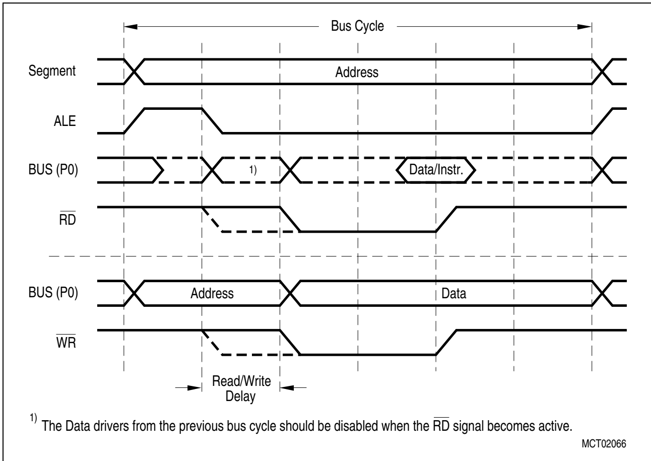
Figure 51 Read/Write Delay
