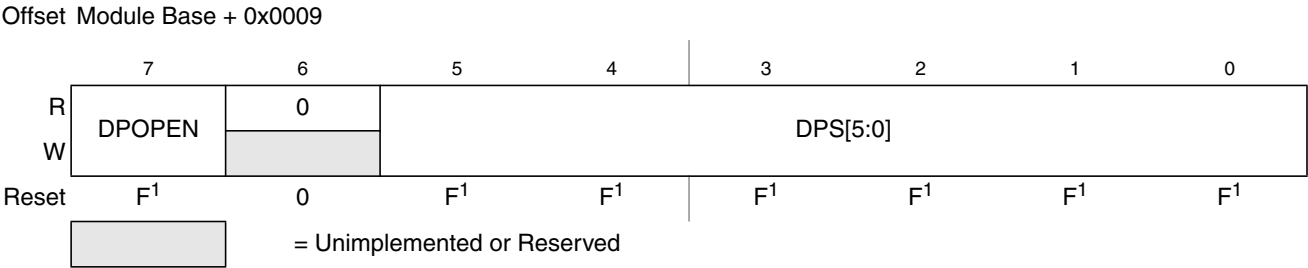
Figure 27-15. EEPROM Protection Register (EEPROT)
