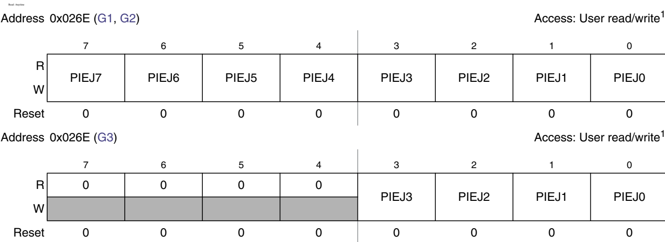
Figure 2-47. Port J Interrupt Enable Register (PIEJ)
