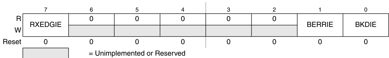
Figure 20-7. SCI Alternative Control Register 1 (SCIACR1)
