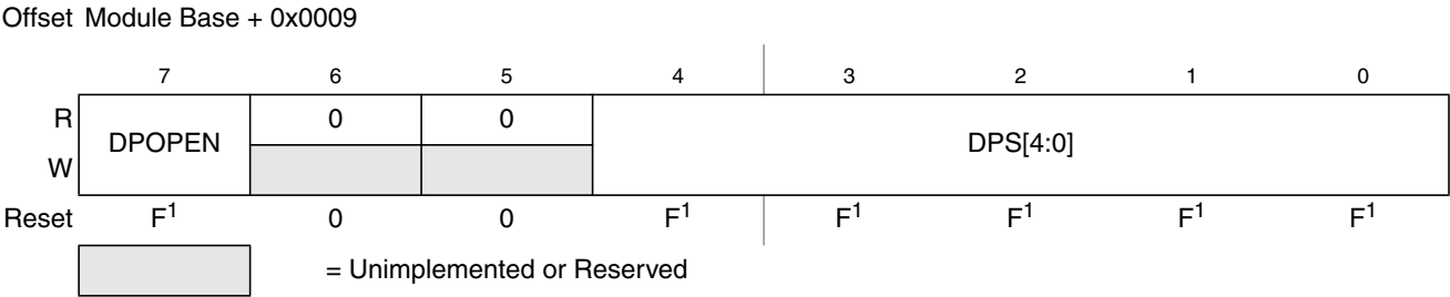
Figure 25-15. EEPROM Protection Register (EEPROT)
