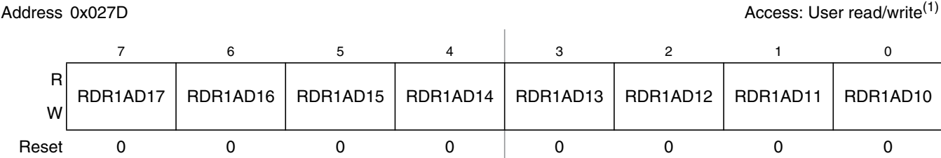
Figure 2-80. Port AD1 Reduced Drive Register 1 (RDR1AD1)
