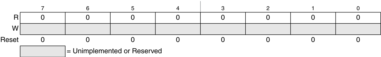
Figure 23-8. Reserved 06
