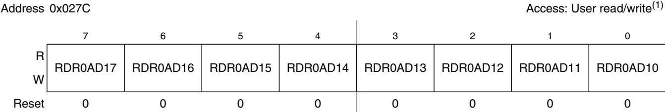
Figure 2-79. Port AD1 Reduced Drive Register 0 (RDR0AD1)
