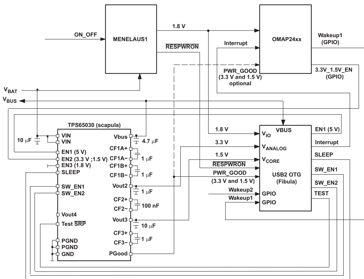
Figure 9. Application Schematic
