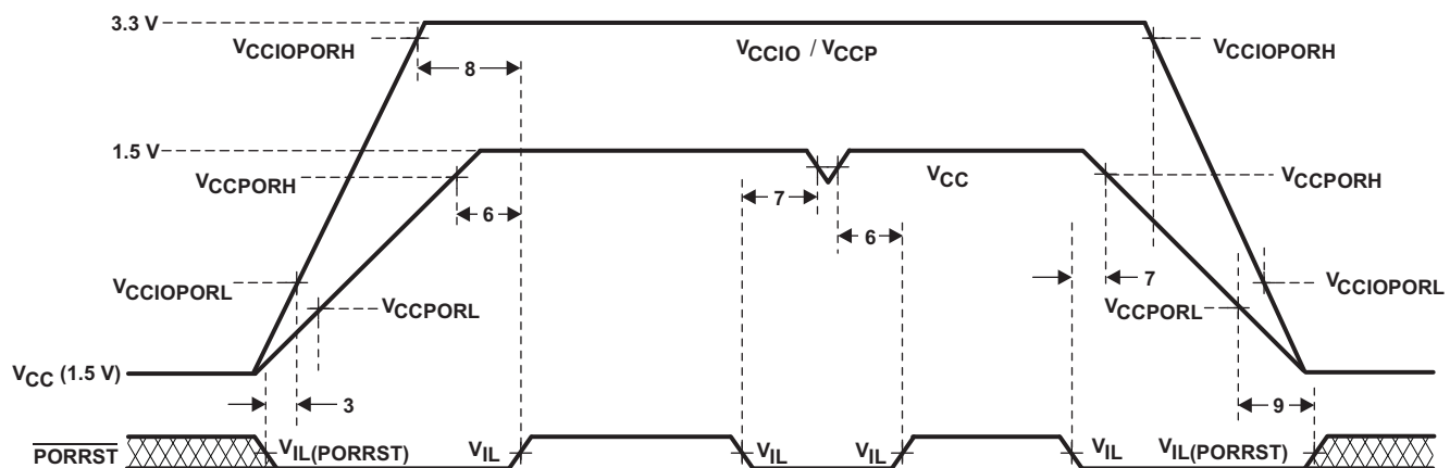
Figure 7-5. \overline{\text{PORRST}} Timing Diagram
