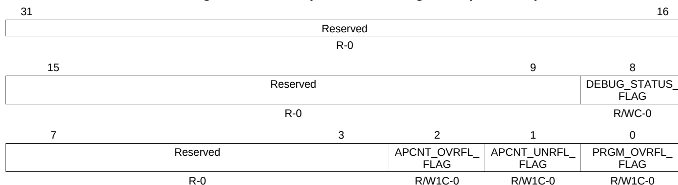
Figure 20-64. Exception Control Register 2 (HETEXC2)
