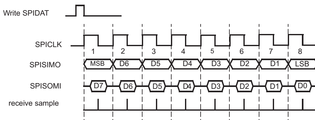
Figure 24-8. Clock Mode with Polarity = 0 and Phase = 0
