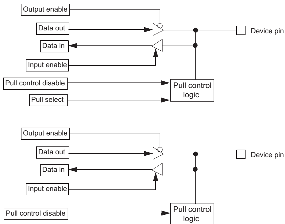
Figure 26-32. GPIO Functionality
