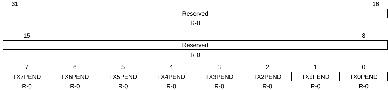
Figure 28-48. Transmit Interrupt Status (Unmasked) Register (TXINTSTATRAW)
