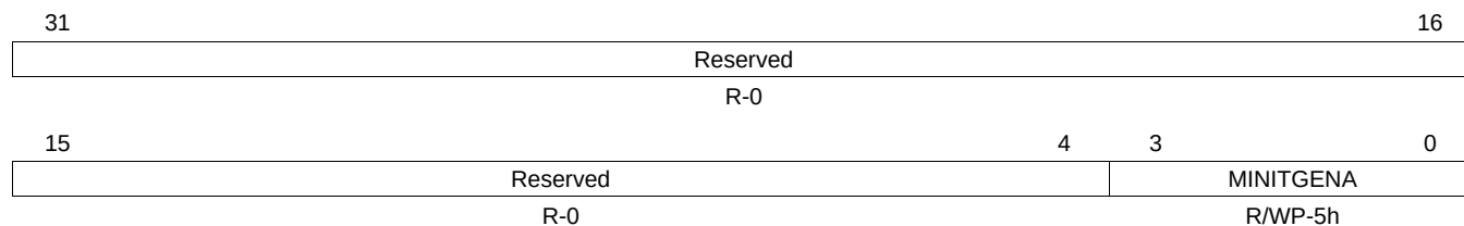
Figure 2-26. Memory Hardware Initialization Global Control Register (MINITGCR) [offset = 5Ch]
