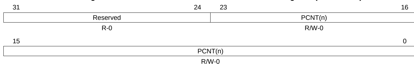
Figure 20-102. HWAG Current Tooth Period Value Register (HWAPCNT)
