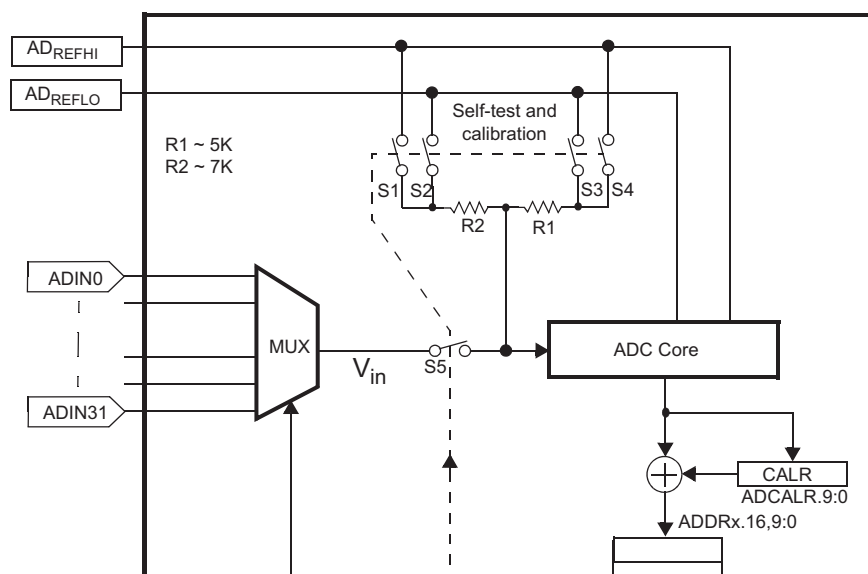
Figure 19-11. Self-Test and Calibration Logic
