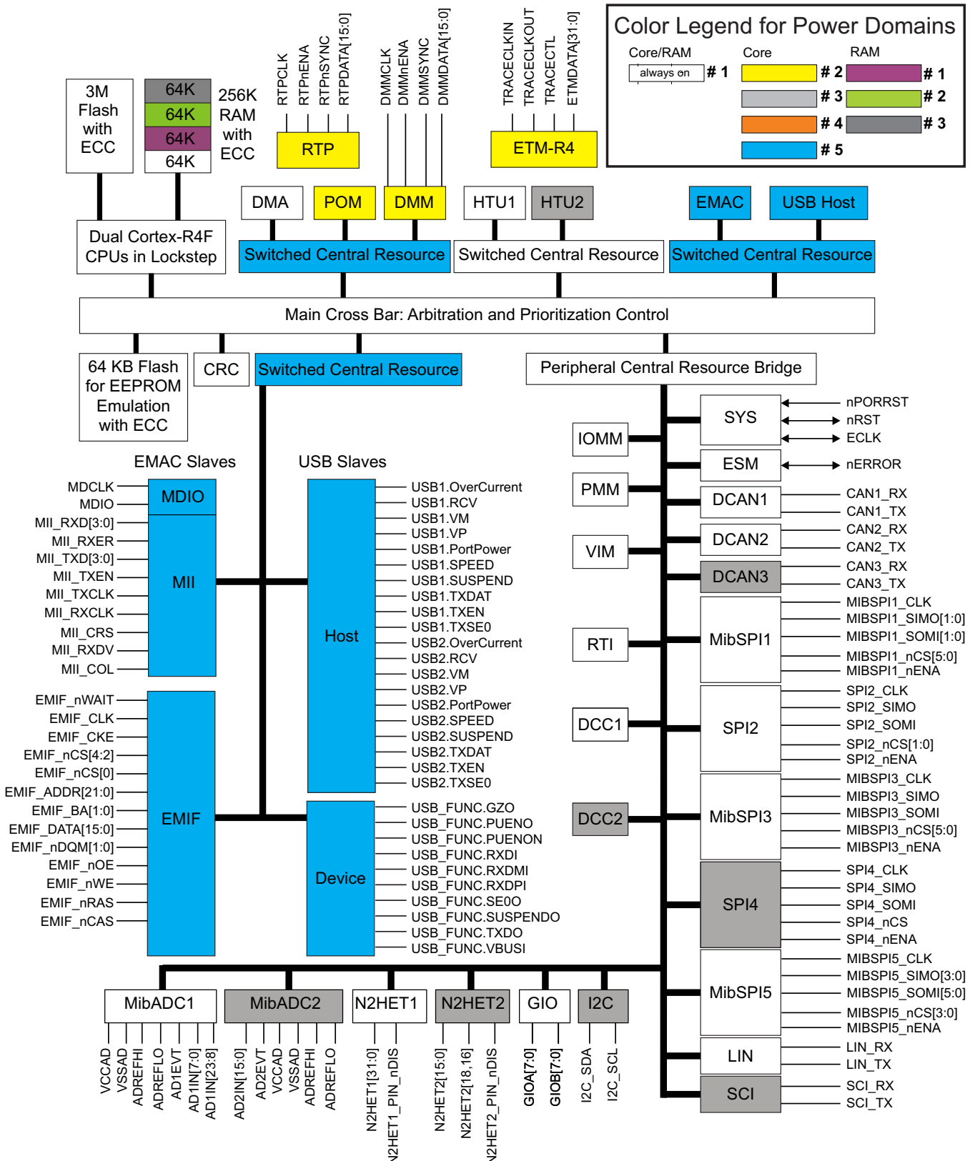
Figure 1-1. Block Diagram
