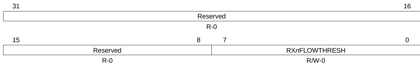
Figure 28-68. Receive Channel n Flow Control Threshold Register (RX n FLOWTHRESH)
