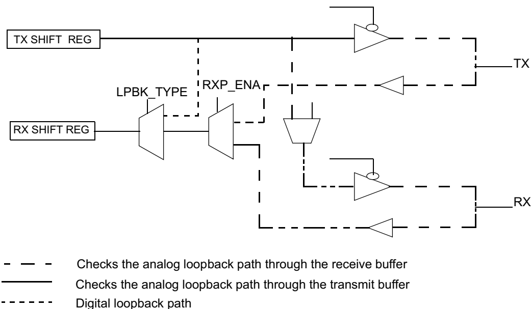
Figure 24-22. I/O Paths during I/O Loopback Modes
