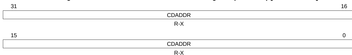
Figure 16-87. Current Destination Address Register (CDADDR) [offset = 804h]
