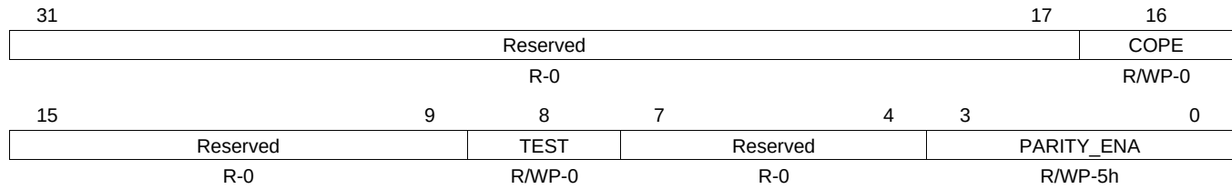
Figure 21-37. Parity Control Register (HTU PCR) [offset = 64h]
