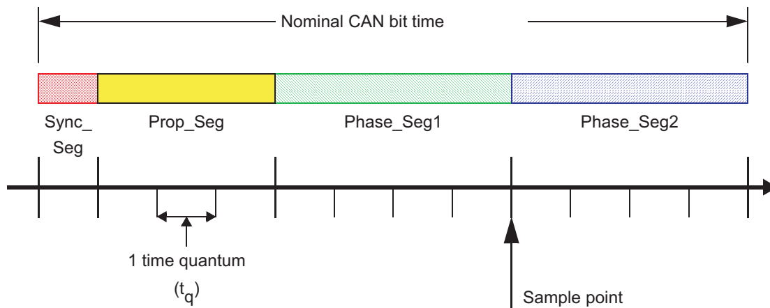
Figure 23-2. Bit Timing
