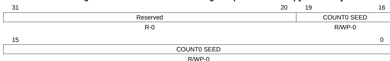
Figure 11-9. DCC Counter0 Seed Register (DCCCNT0SEED) [offset = 8h]
