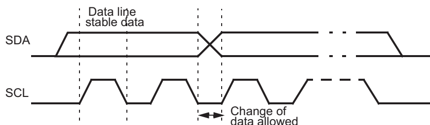
Figure 27-4. Bit Transfer on the I2C Bus
