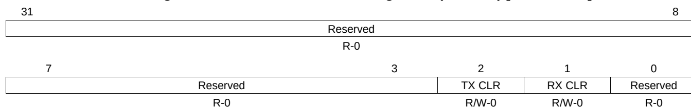
Figure 25-47. SCI Pin I/O Control Register 5 (SCIPIO5) [offset = 50h]
