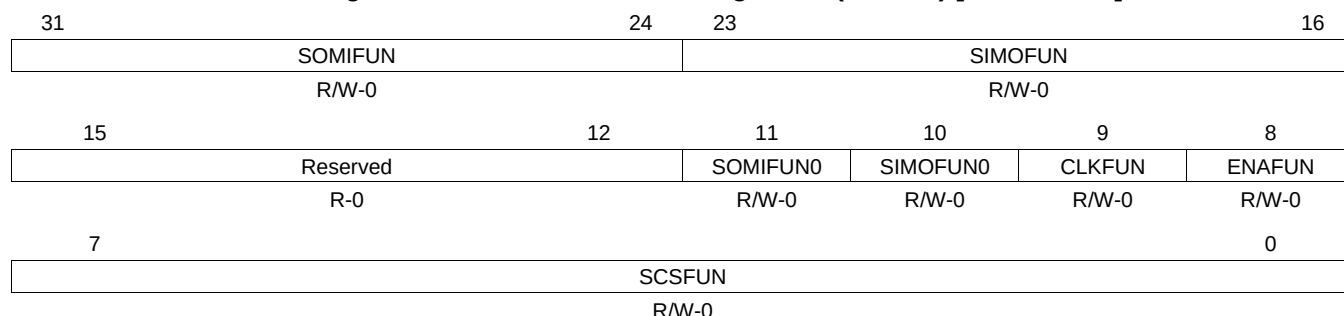
Figure 24-31. SPI Pin Control Register 0 (SPIPC0) [offset = 14h]
