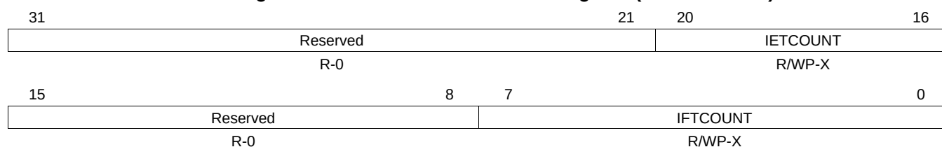
Figure 21-45. Initial Transfer Count Register (HTU ITCOUNT)
