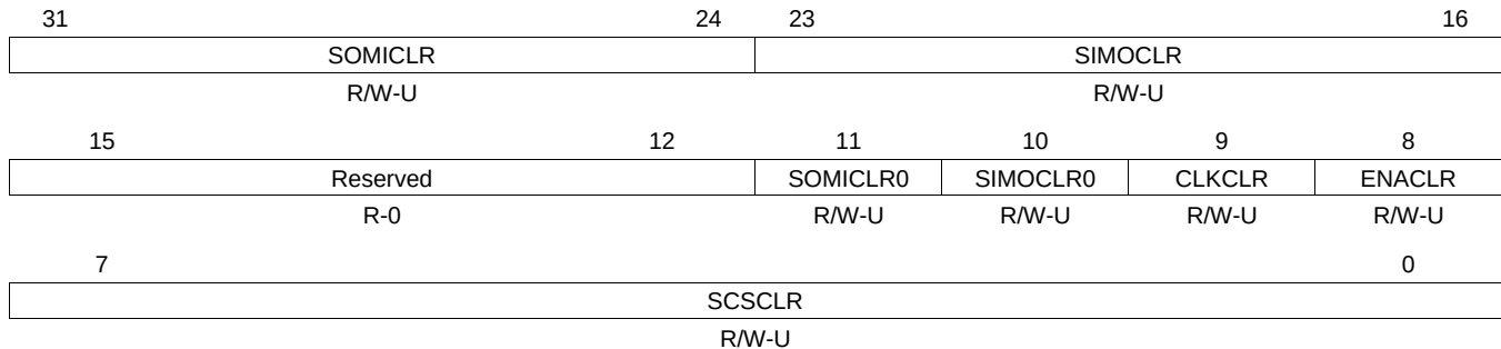
Figure 24-36. SPI Pin Control Register 5 (SPIPC5) [offset = 28h]
