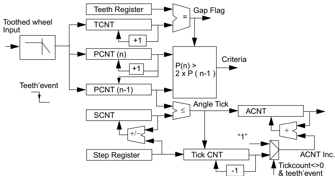
Figure 20-38. New Angle Tick Generation Architecture
