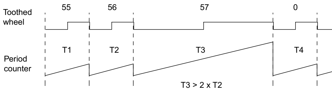
Figure 20-45. Gap Verification Criteria For a 60-2 Toothed Wheel
