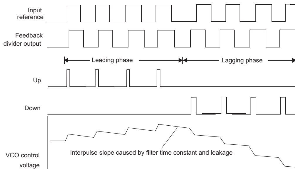
Figure 10-10. PFD Timing
