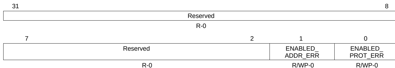
Figure 4-9. ERR_ENABLED_STATUS_REG: Error Enabled Status / Clear Register (Address = FFFFEAE4h)
