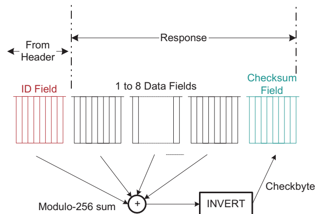
Figure 25-23. LIN 2.0-Compliant Checksum Generation at Transmitting Node
