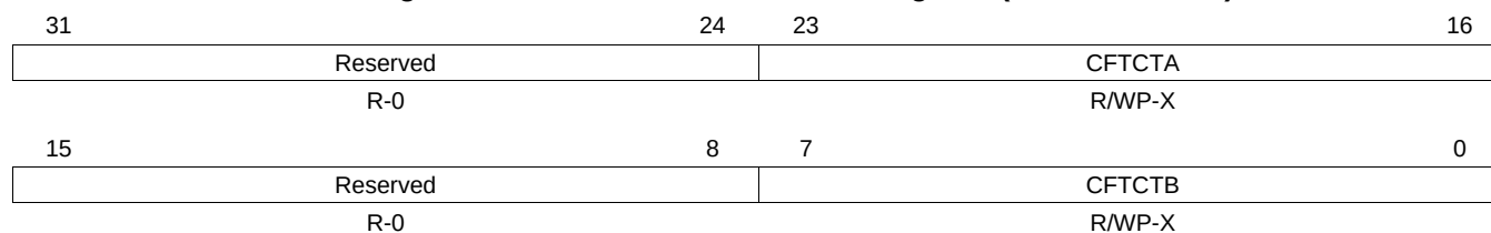
Figure 21-48. Current Frame Count Register (HTU CFCOUNT)
