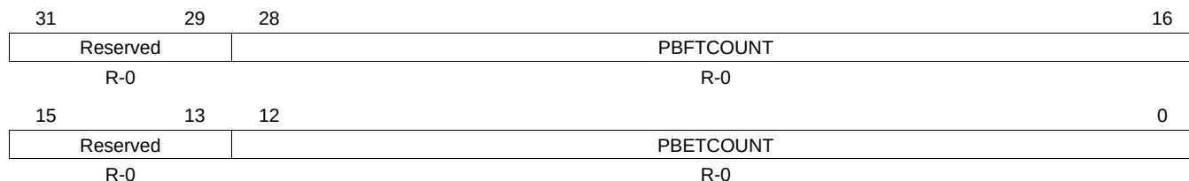
Figure 16-67. Port B Active Channel Transfer Count Register (PBACTC) [offset = 1A0h]
