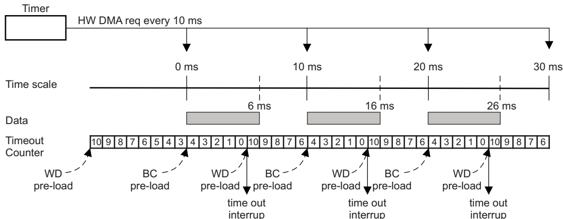
Figure 14-7. Timeout Example 2
