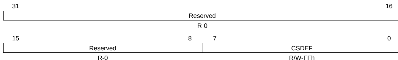
Figure 24-49. SPI Default Chip Select Register (SPIDEF) [offset = 4Ch]
