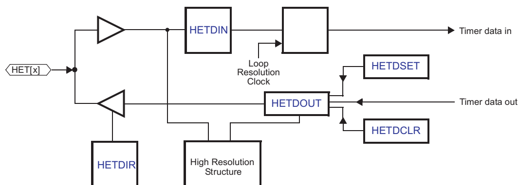
Figure 20-8. I/O Control
