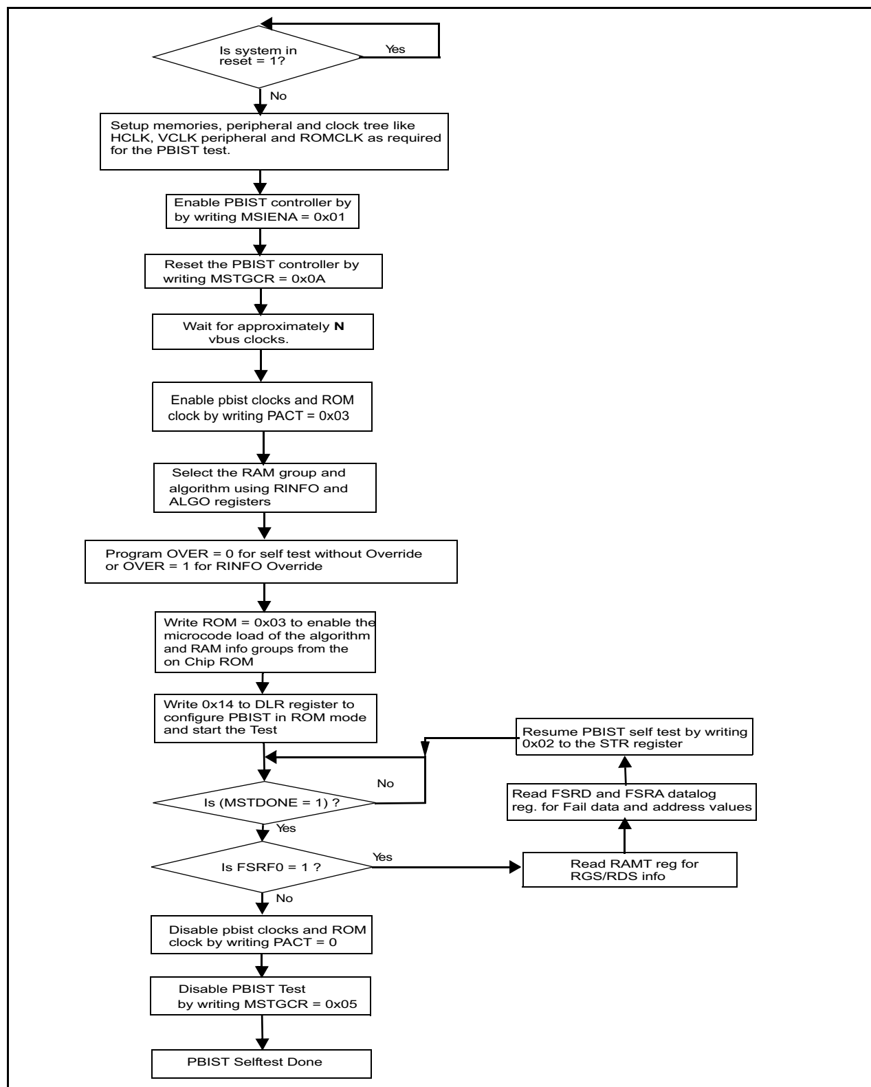
Figure 7-2. PBIST Memory Self-Test Flow Diagram
