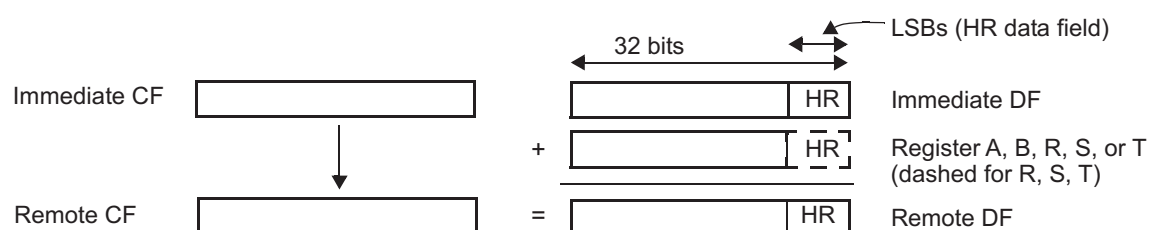
Figure 20-173. RADM64 Add and Move Operation
