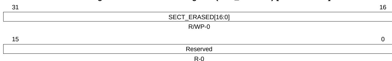
Figure 5-40. FSM Sector Register (FSM_SECTOR) [offset = 2A4h]
