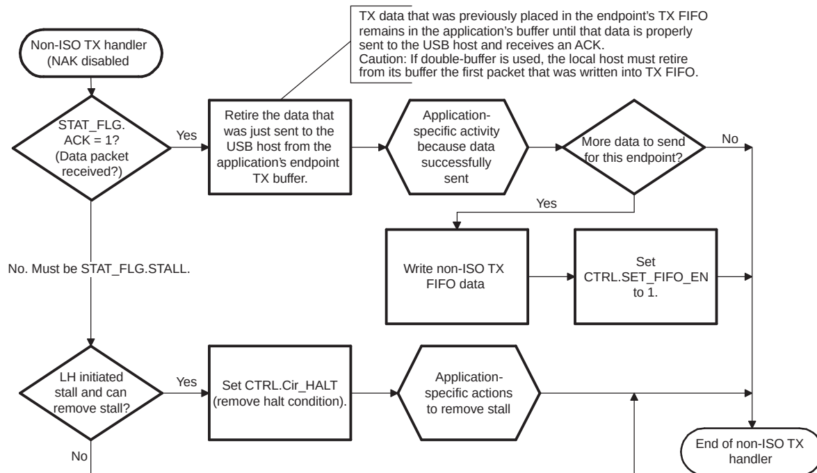
Figure 29-79. Non-Isochronous Non-Control Endpoint Transmit Interrupt Handler
