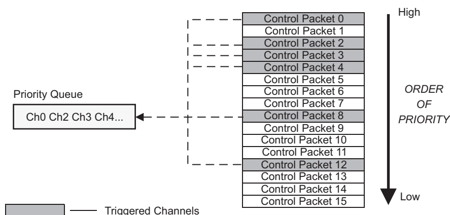
Figure 16-9. Fixed Priority Scheme
