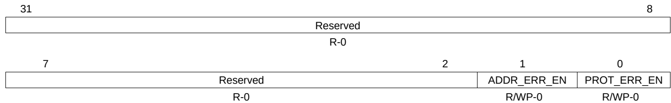
Figure 4-10. ERR_ENABLE_REG: Error Signaling Enable Register (Address = FFFFEAE8h)
