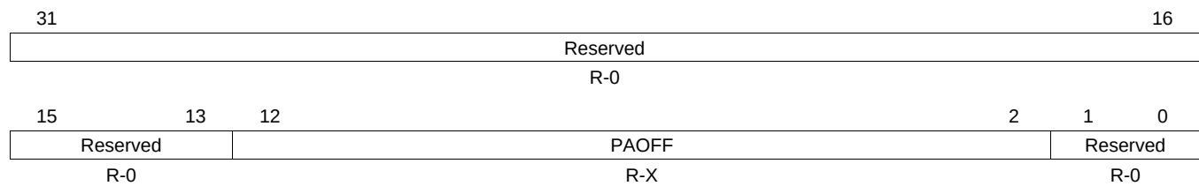
Figure 20-82. Parity Address Register (HETPAR)
