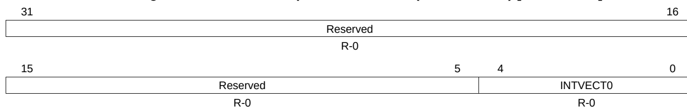
Figure 25-35. SCI Interrupt Vector Offset 0 (SCIINTVECT0) [offset = 20h]
