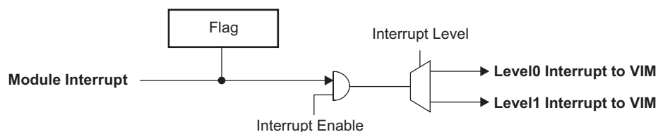
Figure 30-6. Interrupt Structure
