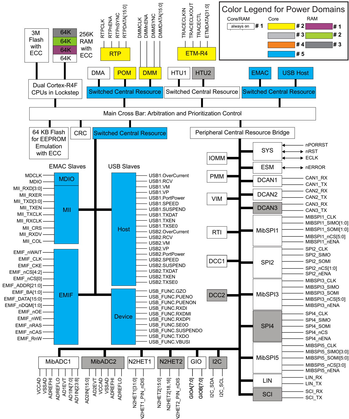
Figure 3-2. Core Power Domains
