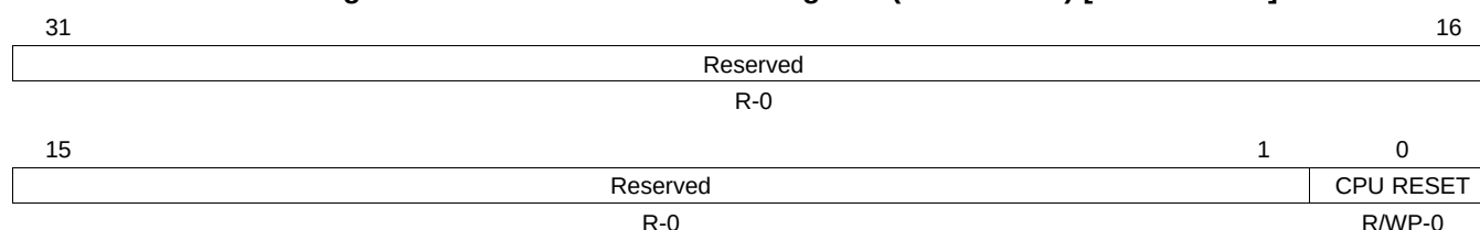
Figure 2-48. CPU Reset Control Register (CPURSTCR) [offset = CCh]
