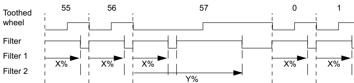
Figure 20-48. Filtering During Singularity Tooth
