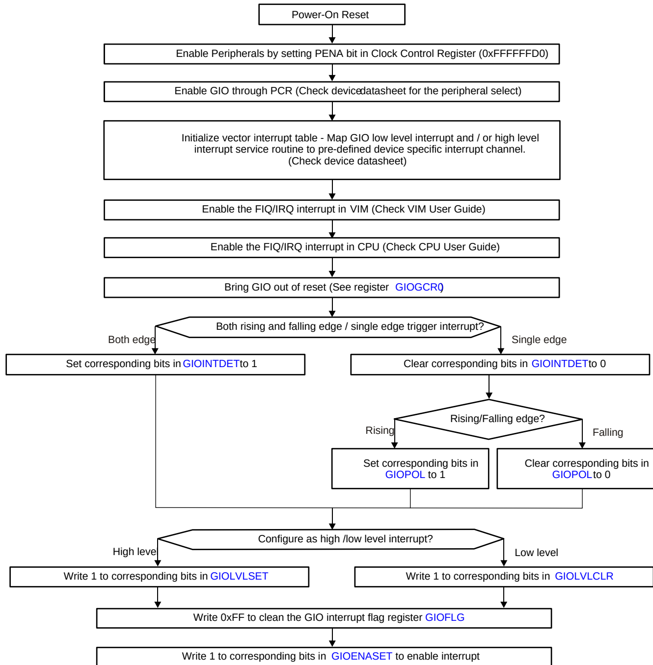
Figure 22-2. Interrupt Generation Function Quick Start Flow Chart
