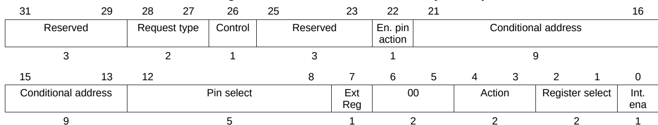
Figure 20-145. ECMP Control Field (C31:C0)
