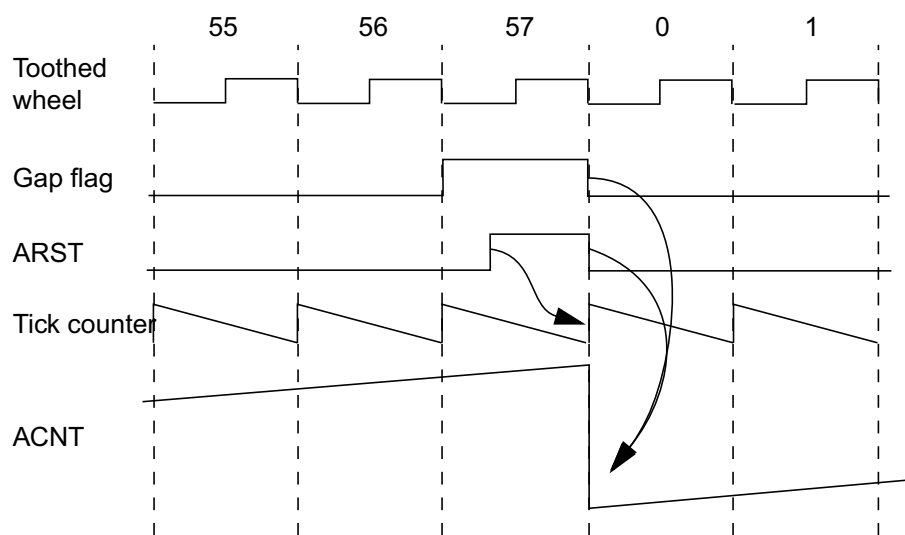
Figure 20-46. Using the ARST Bit in a Toothed Wheel Without Singularity
