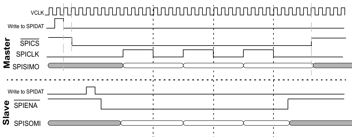
Figure 24-84. SPI/MibSPI Pins During Master/Slave Mode with 5-pin Configuration
