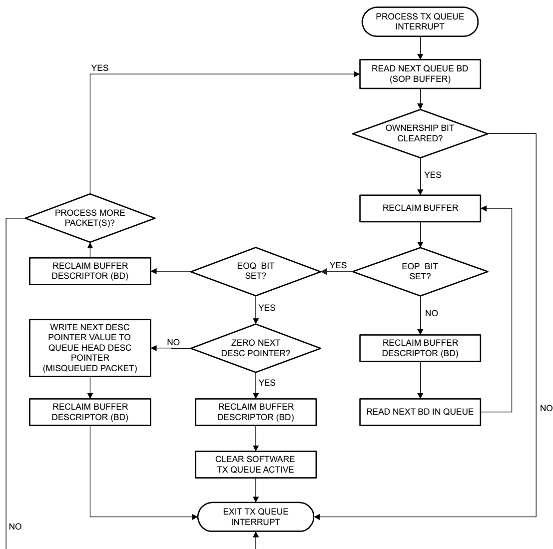
Figure 28-9. Transmit Queue Interrupt Processing Flow Chart
