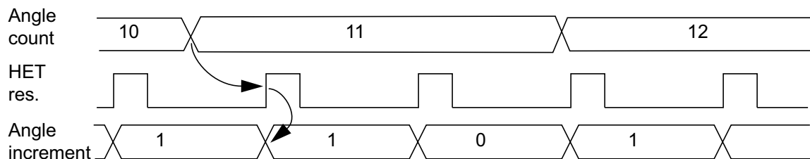
Figure 20-51. Angle Count Within the HWAG at Resolution Clock
