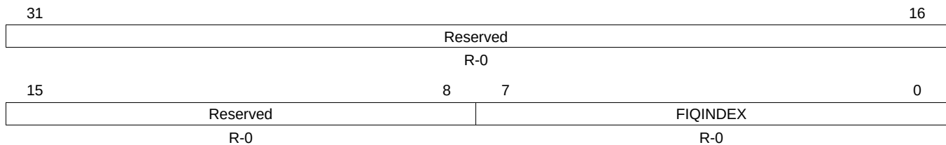
Figure 15-16. FIQ Index Offset Vector Register (FIQINDEX) [offset = 04h]
