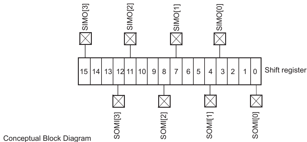
Figure 24-18. 4-Data Line Mode (Phase 0, Polarity 0)
