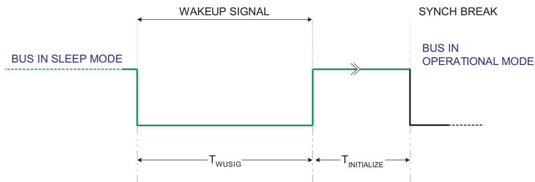
Figure 25-26. Wakeup Signal Generation
