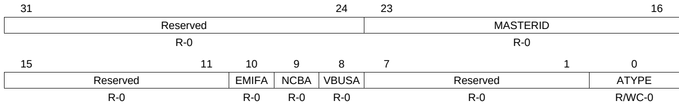
Figure 2-40. Imprecise Fault Status Register (IMPFSTS) [offset = A8h]
