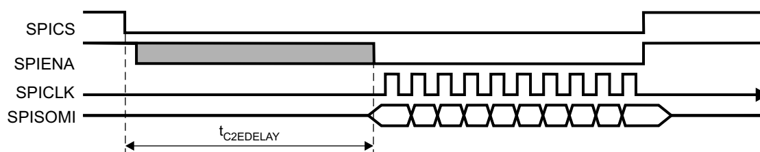
Figure 24-48. Chip-Select-Active-to-ENA-Signal-Active-Timeout
