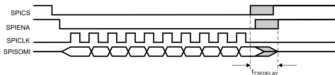
Figure 24-47. Transmit-Data-Finished-to-ENA-Inactive-Timeout
