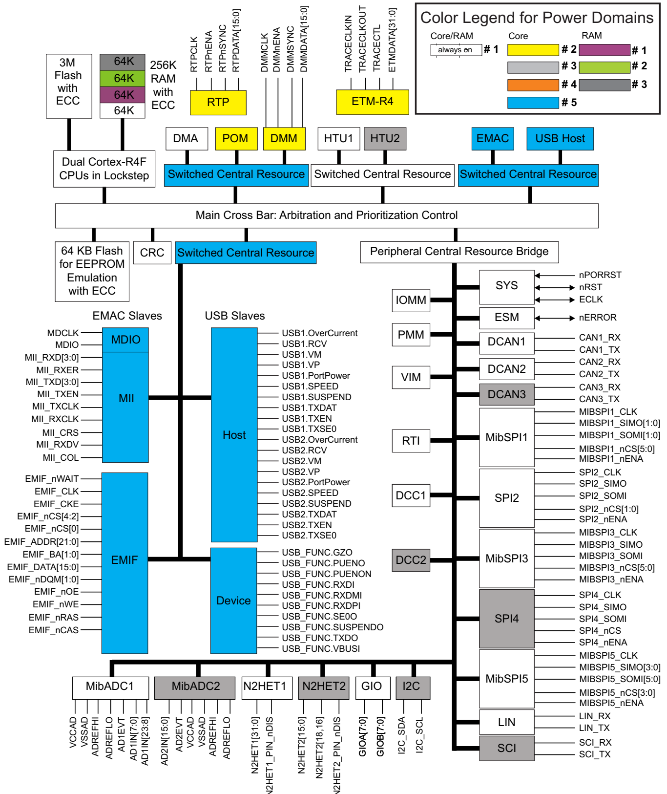
Figure 1-1. Block Diagram
