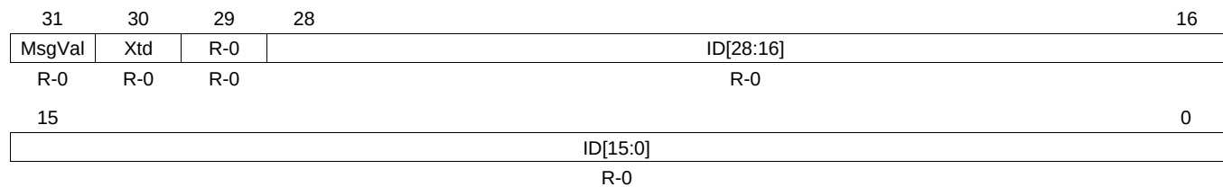
Figure 23-66. IF3 Arbitration Register (DCAN IF3ARB) [offset = 148h]
