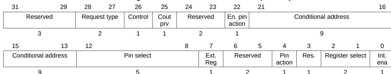
Figure 20-110. ACMP Control Field (C31:C0)
