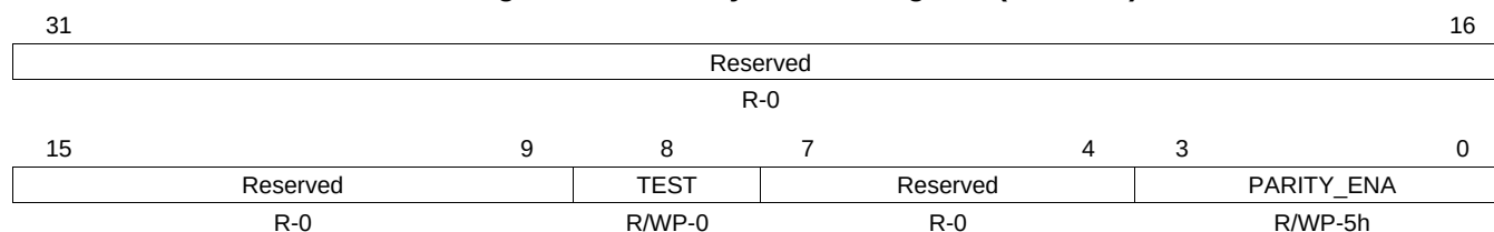
Figure 20-81. Parity Control Register (HETPCR)
