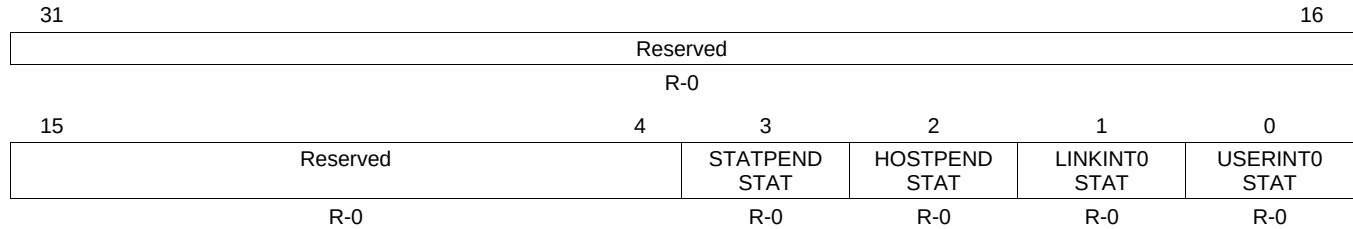
Figure 28-25. EMAC Control Module Miscellaneous Interrupt Status Register (C0MISCSTAT)
