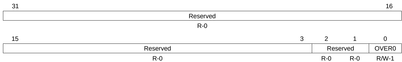
Figure 7-7. Override Register (OVER) [offset = 0188h]
