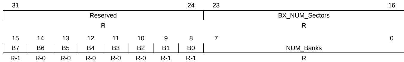
Figure 5-2. TI OTP Bank 0 Sector Information
