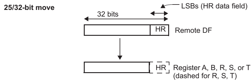
Figure 20-159. MOV32 Move Operation for REMTOREG (Case 11)
