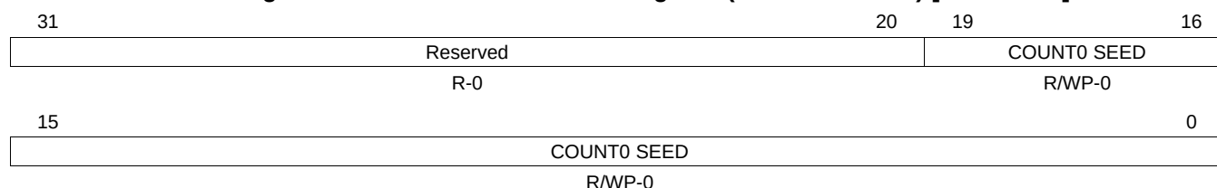
Figure 11-9. DCC Counter0 Seed Register (DCCCNT0SEED) [offset = 8h]
