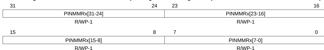
Figure 4-15. PINMMRnn: Pin Multiplexing Control Registers (Address = FFFFEB10h-FFFFEB88h)
