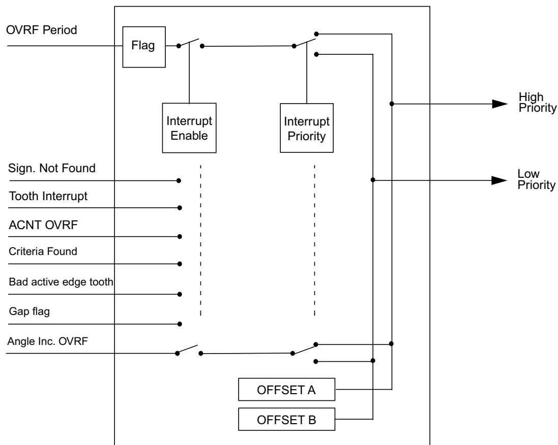
Figure 20-49. HWAG Interrupt Block Diagram
