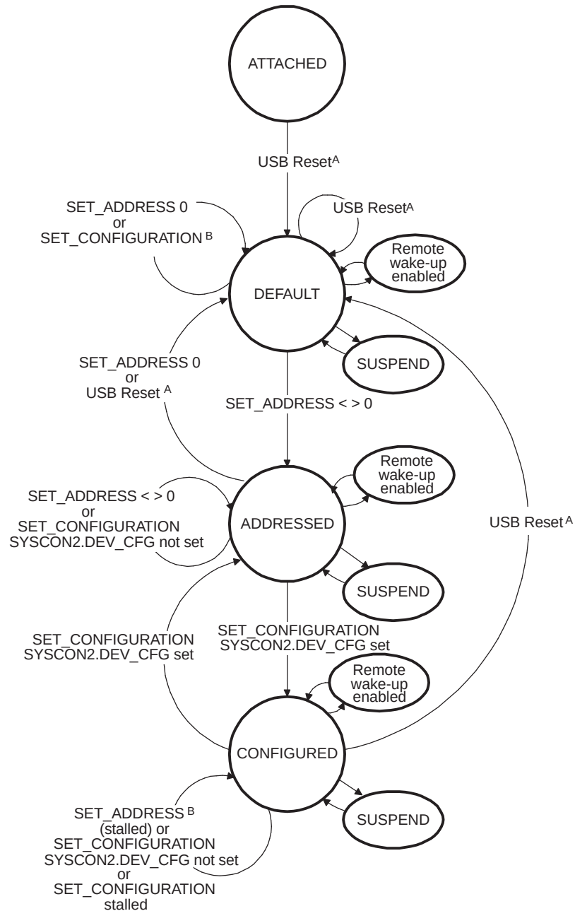
Figure 29-69. USB Device Controller Device State Transitions
