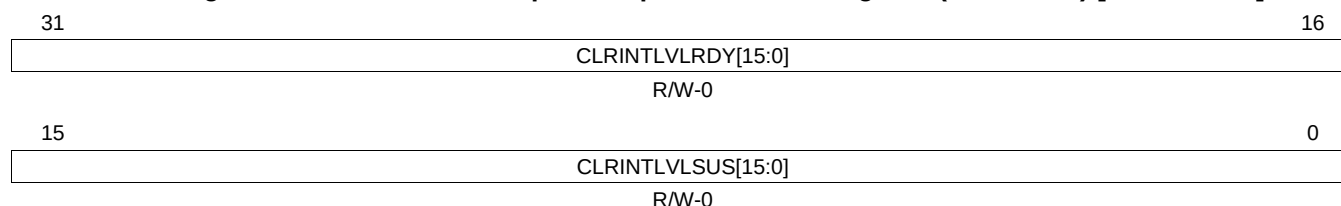
Figure 24-59. Transfer Group Interrupt Level Clear Register (TGITLVCR) [offset = 80h]
