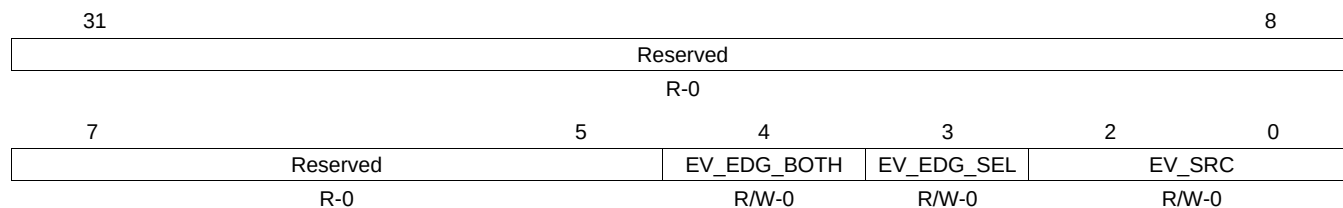
Figure 19-28. ADC Event Group Trigger Source Select Register (ADEVSRC) [offset = 1Ch]
