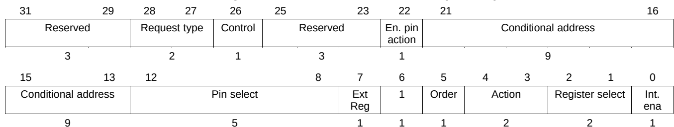
Figure 20-151. MCMP Control Field (C31:C0)
