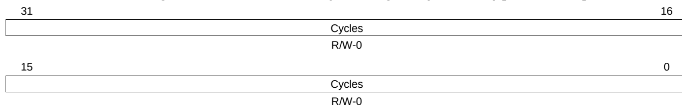
Figure 32-5. EFC Self Test Cycles Register (EFCSTCY) [offset = 48h]
