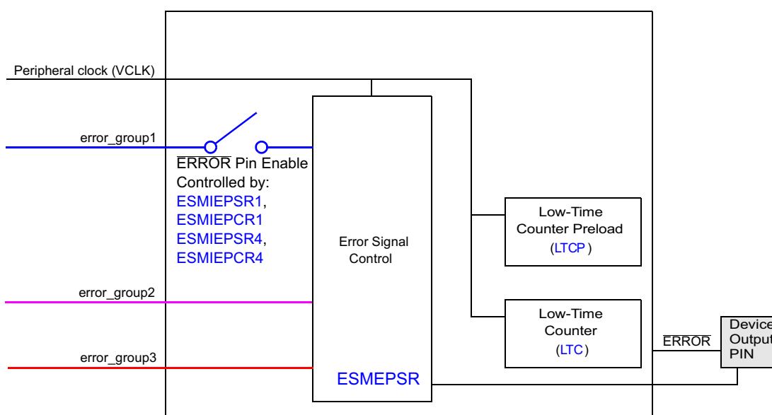
Figure 12-3. \overline{\text{ERROR}} Pin Response Handling
