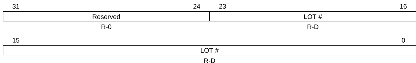
Figure 2-34. Die Identification Register, Upper Word (DIEIDH) [offset = 80h]
