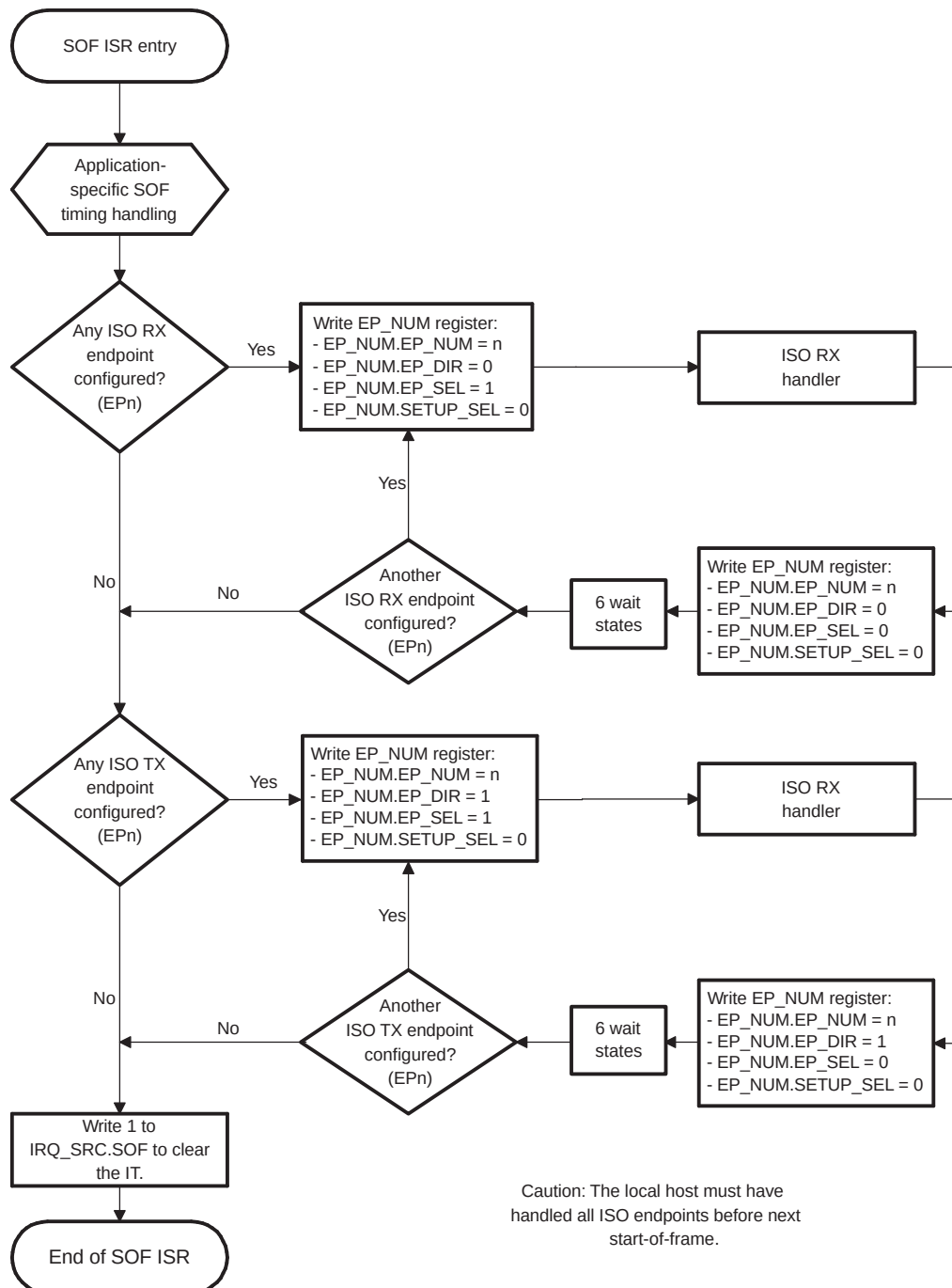
Figure 29-81. SOF Interrupt Handler Flowchart
