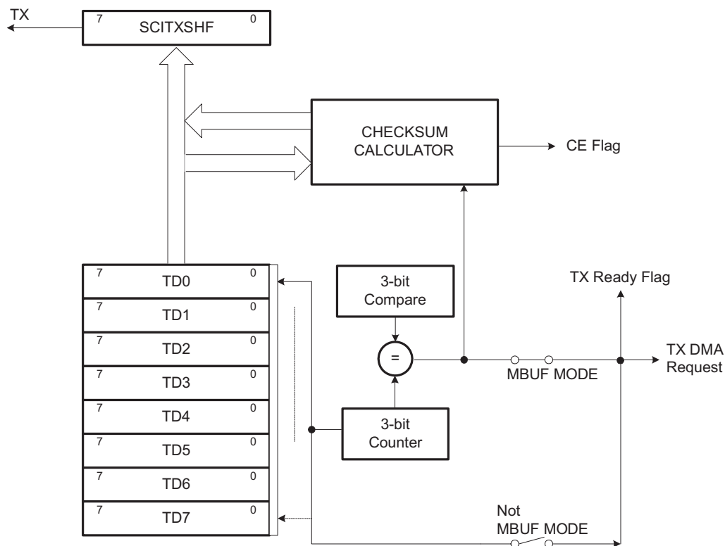
Figure 25-9. Transmit Buffers
