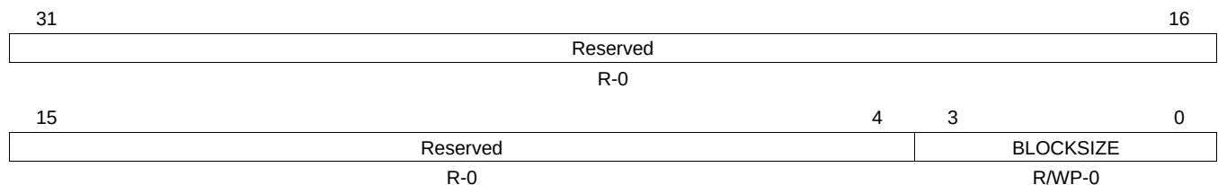
Figure 30-15. DMM Direct Data Mode Blocksize Register (DMMDDMBL) [offset = 20h]
