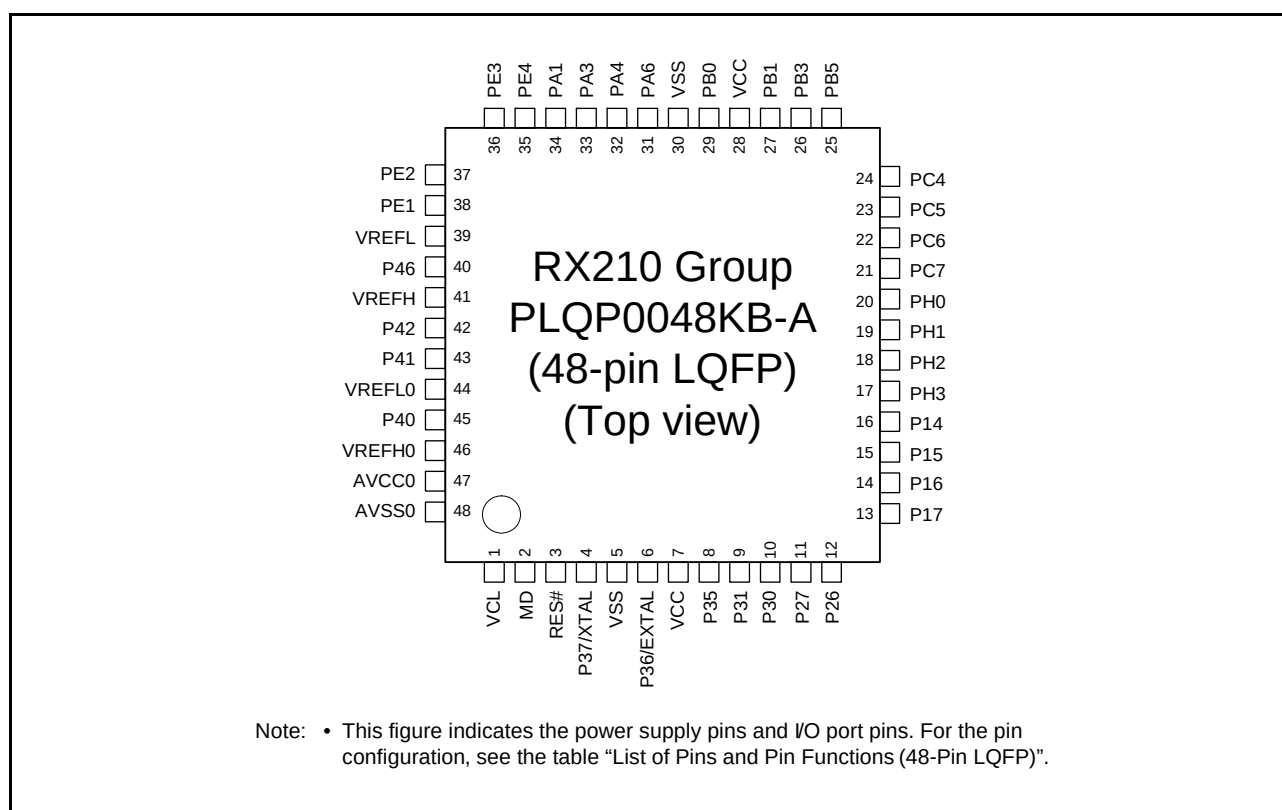
Figure 1.11 Pin Assignments of the 48-Pin LQFP
