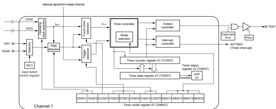
Figure 3-5. Internal Block Diagram of Channel 7 of Timer Array Unit 0
