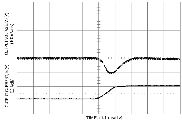
Figure 17. Transient Response to Step Increase in Load from 50% to 75% of Full Load ( V_I = 48 Vdc).
