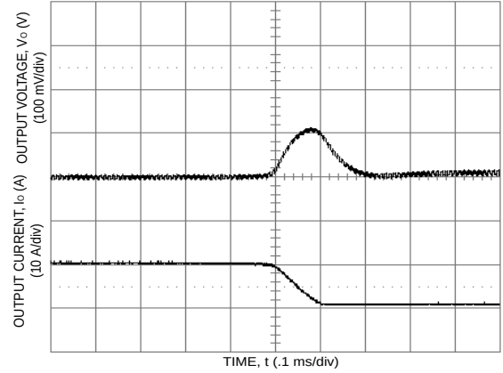
Figure 16. Transient Response to Step Decrease in Load from 50% to 25% of Full Load ( V_I = 48 Vdc).
