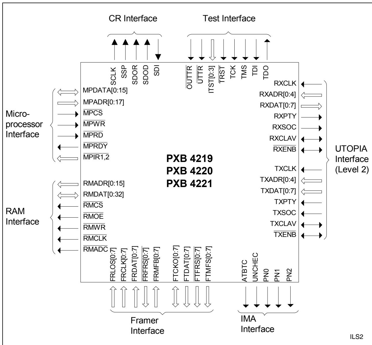
Figure 1 Logic Symbol
