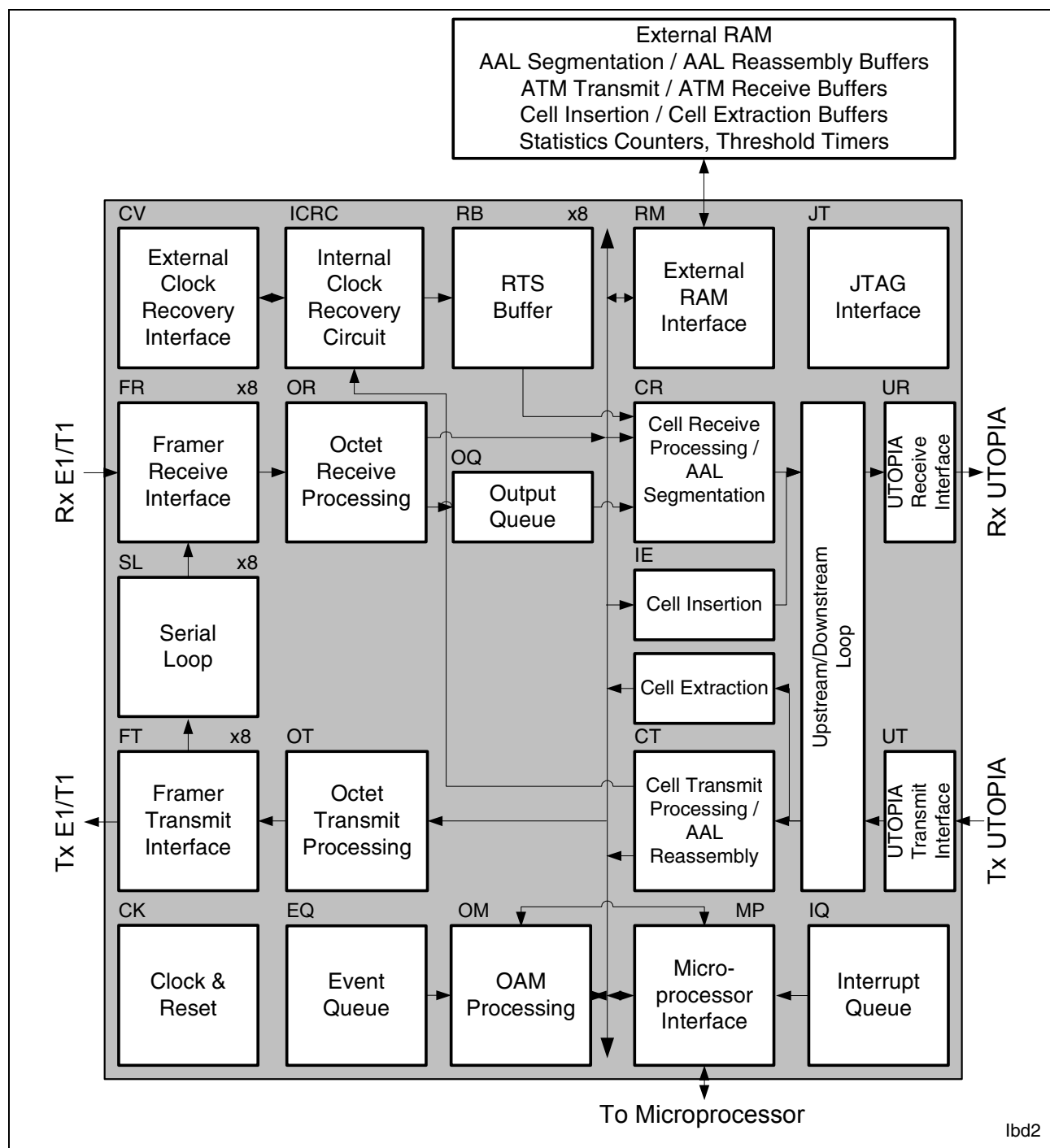
Figure 6 Block Diagram
