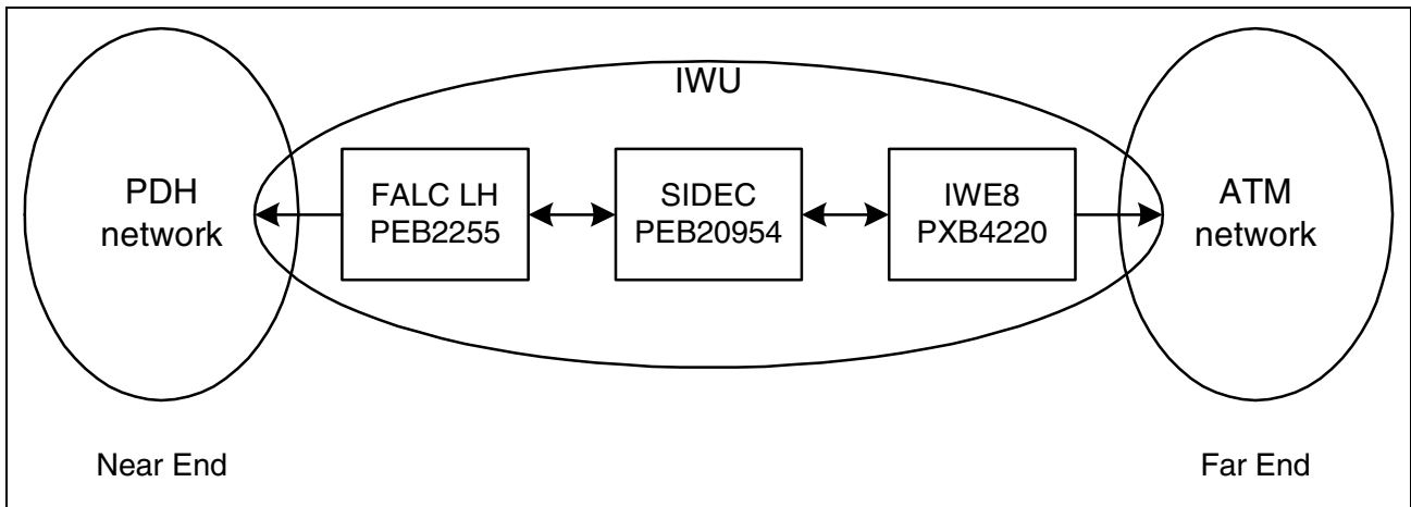
Figure 4 Echo Cancellation Application
