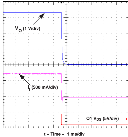
Figure 11. Power Down
