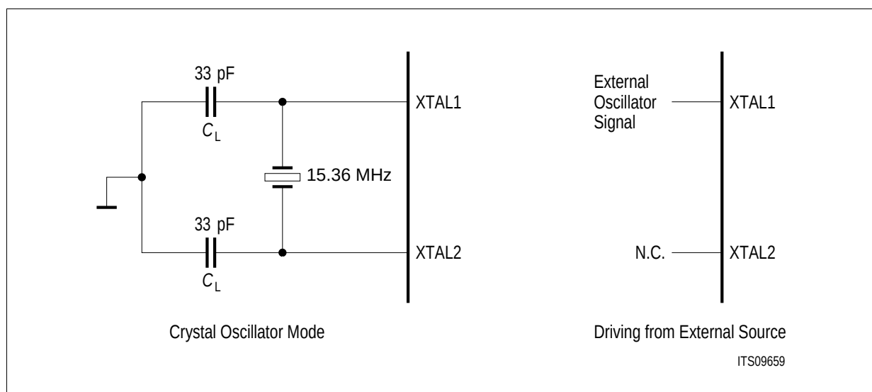
Figure 83 Oscillator Circuit
