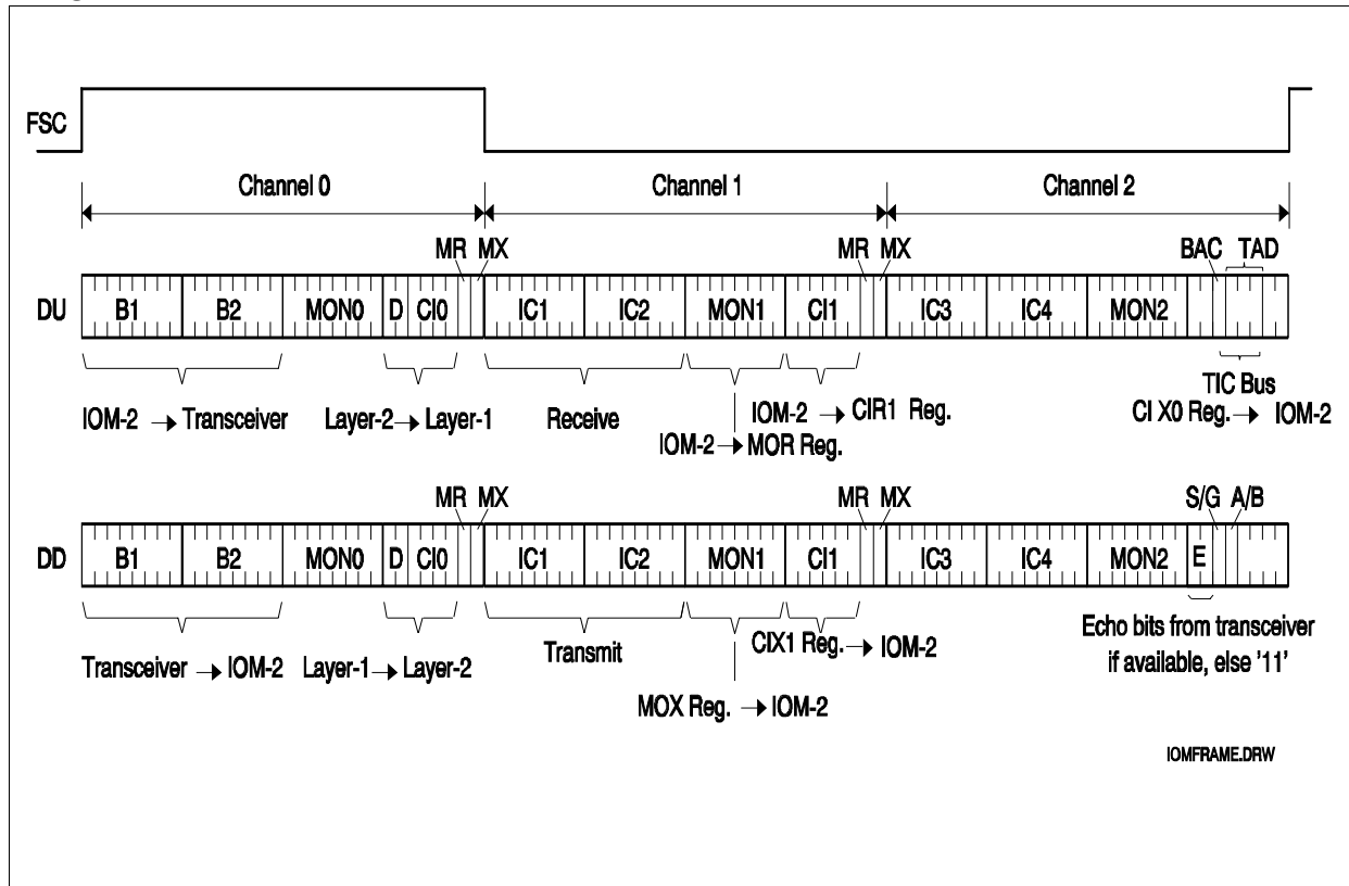
Figure 14 IOM ® -2 Frame Structure in Terminal Mode
