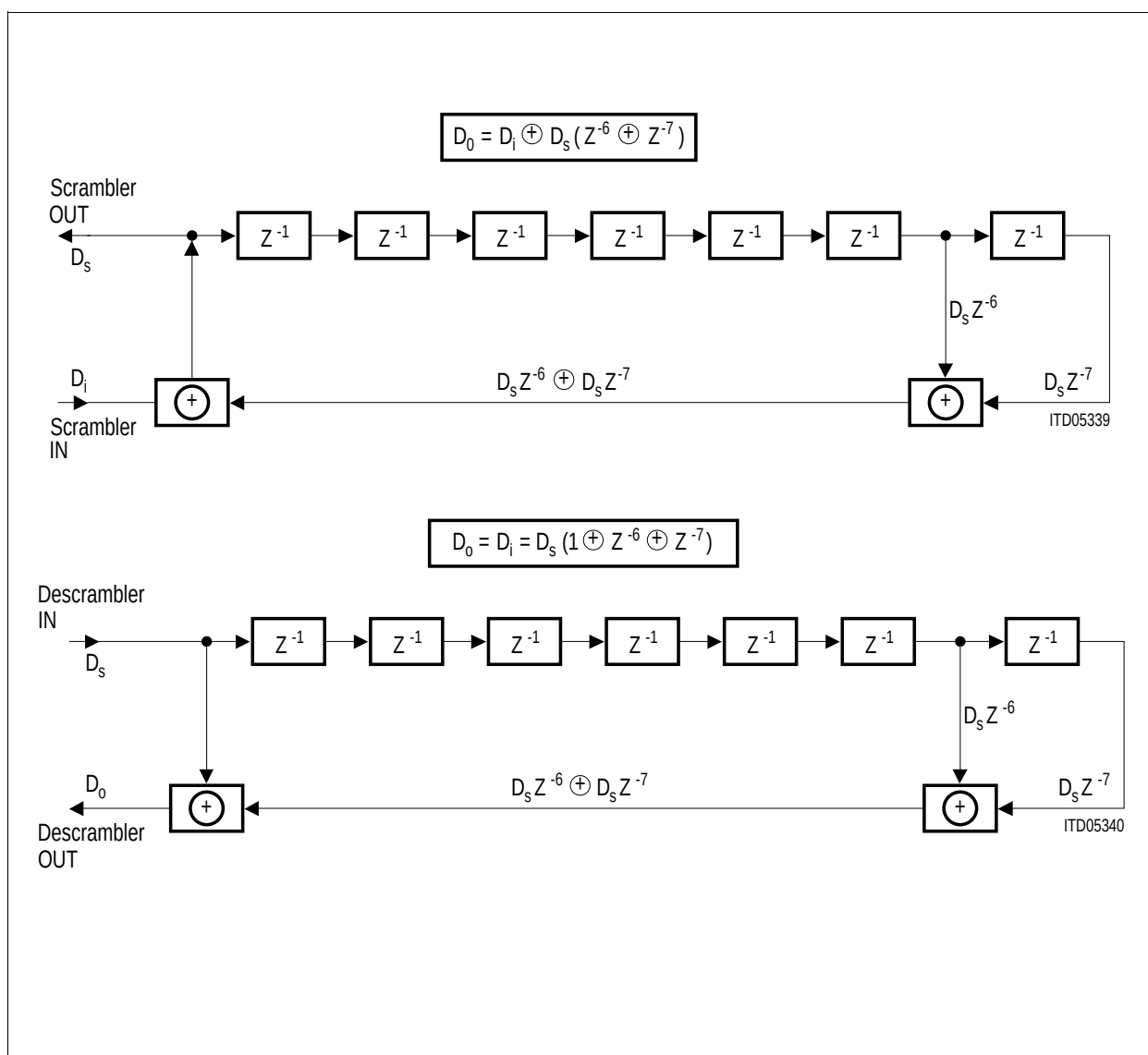
Figure 38 Scrambler/Descrambler
