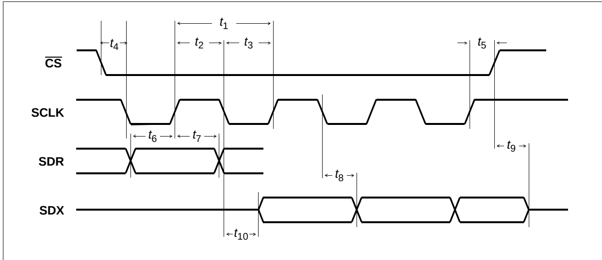
Figure 87 SCI Interface
