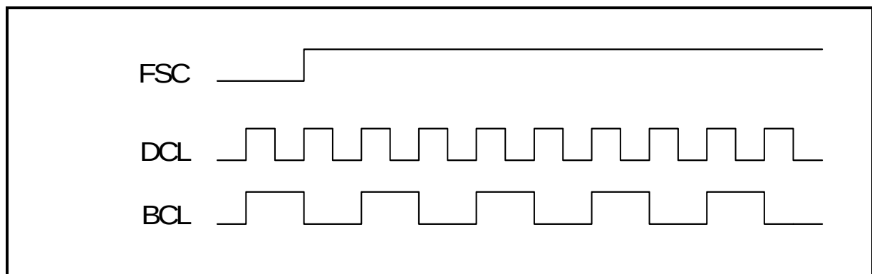
Figure 13 Clock waveforms
