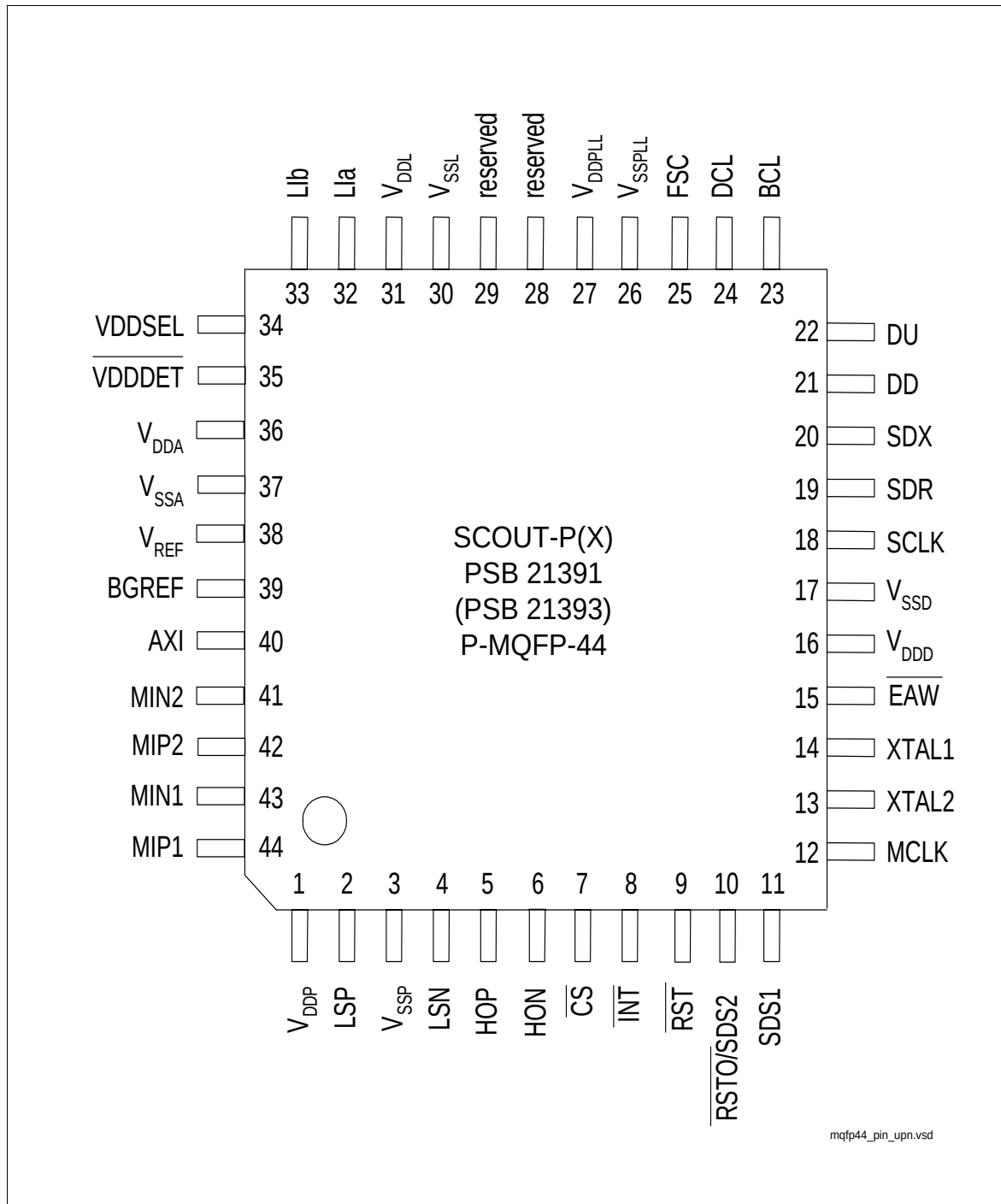
Figure 1 Pin Configuration
