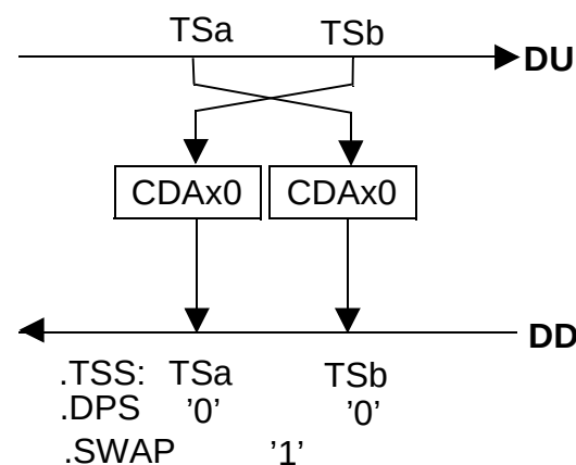
Figure 17 Examples for Data Access via CDAXy Registers
