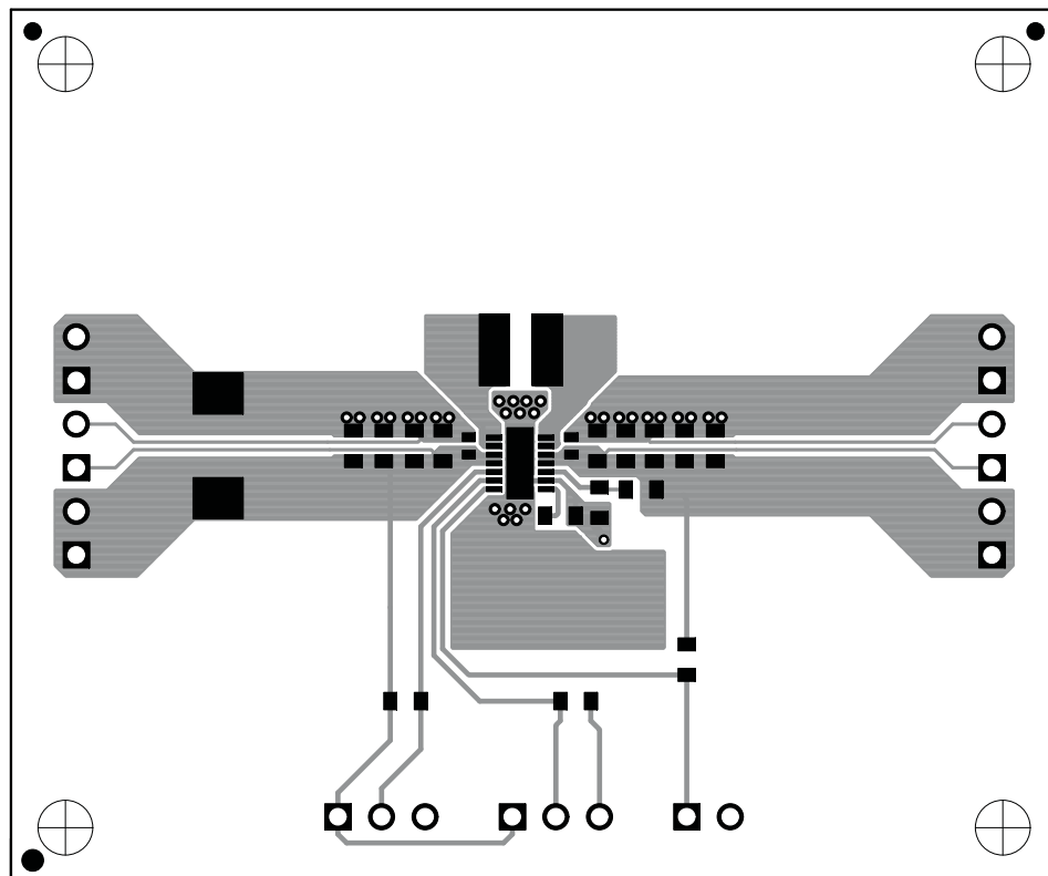
Figure 7. Top Layer Routing
