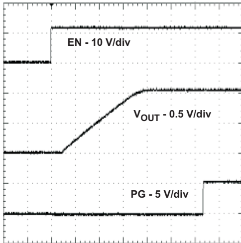
STARTUP WAVEFORM
