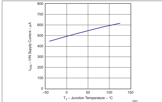
Figure 1. VIN Supply Current vs Junction Temperature
