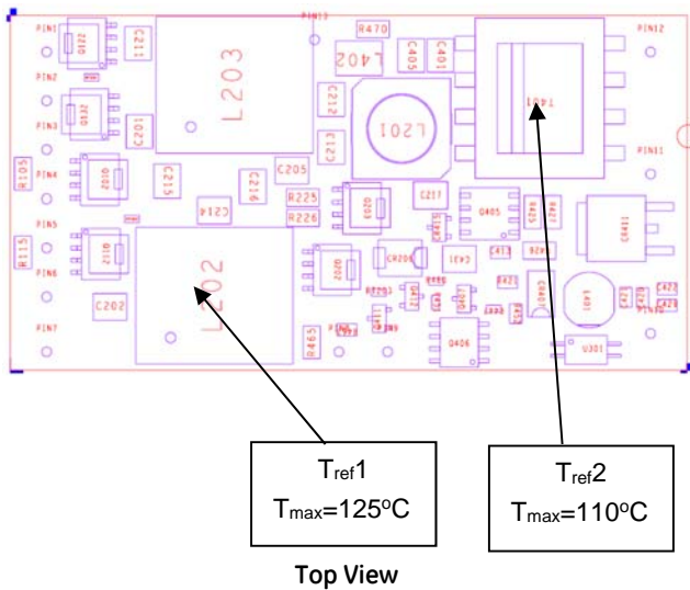
Figure 15. Thermal Reference Point, Tref locations
