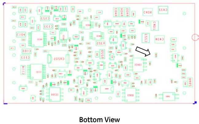
Figure 16. Location of Over Temperature Protection thermal sensors, TOTP (Trip Point = 125°C +/- 5°C)
