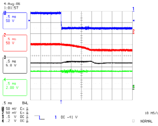
Figure 12. Feeds Switchover Test from -48V_Feed A to -75V_Feed B via Knife Switch
