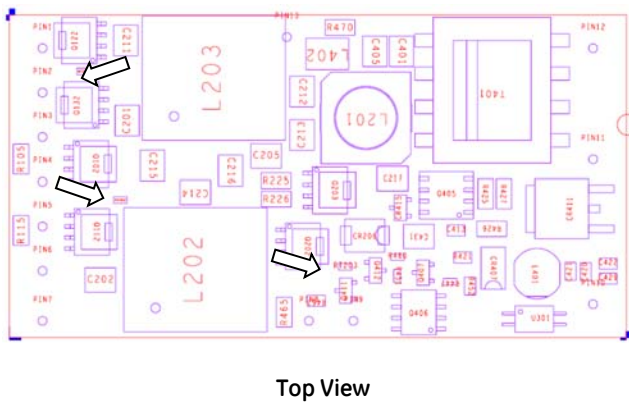
Figure 16. Location of Over Temperature Protection thermal sensors, TOTP (Trip Point = 125°C +/- 5°C)
