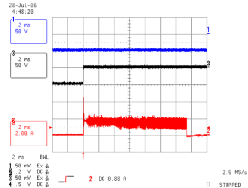
Figure 3. Power Up into Shorted Output CH1: -48_AF, CH3: -48V_OUT, CH2: lin(-48_AF)
