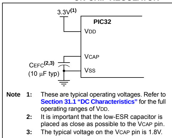
FIGURE 28-1: CONNECTIONS FOR THE ON-CHIP REGULATOR
