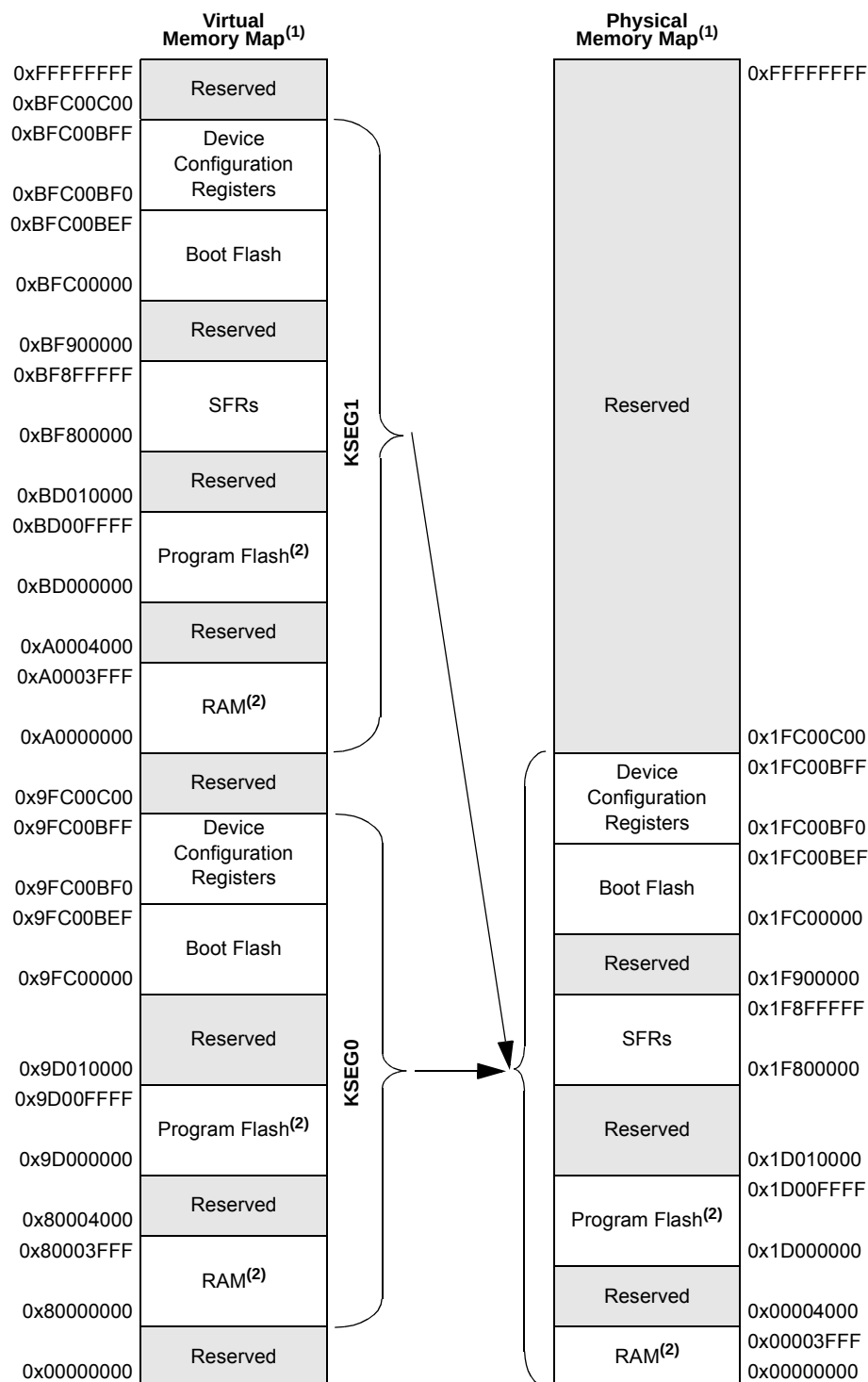
FIGURE 4-3: MEMORY MAP ON RESET FOR PIC32MX130/230 DEVICES (16 KB RAM, 64 KB FLASH)
