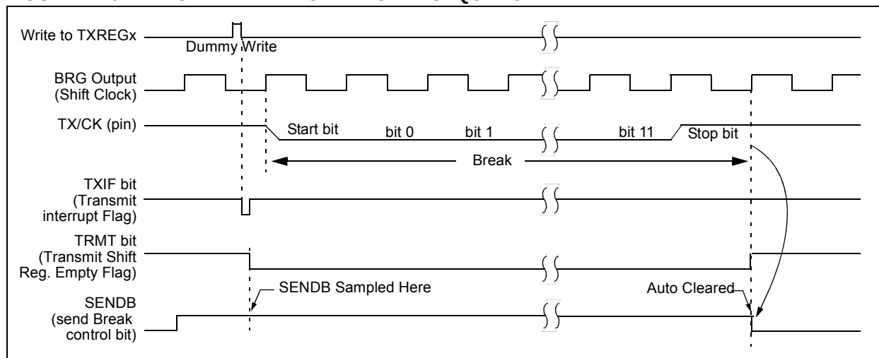
FIGURE 17-9: SEND BREAK CHARACTER SEQUENCE
