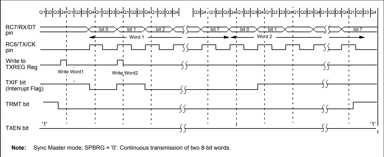
FIGURE 17-6: SYNCHRONOUS TRANSMISSION
