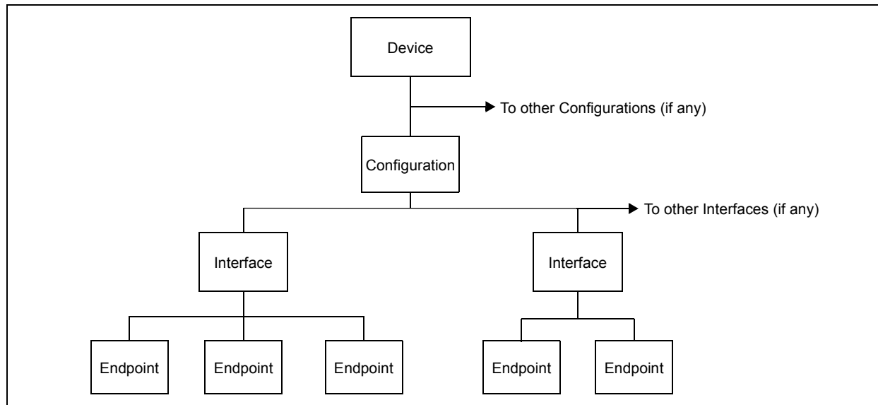
FIGURE 24-12: USB LAYERS
