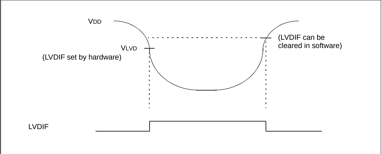
FIGURE 25-3: LOW VOLTAGE DETECT CHARACTERISTICS
